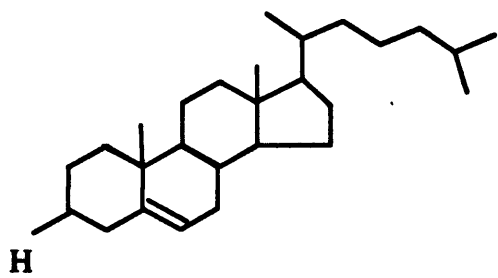
Cholesterol
