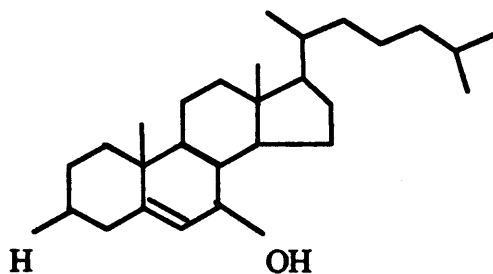
7 \beta -Hydroxycholesterol
