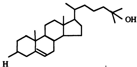
25-Hydroxycholesterol
