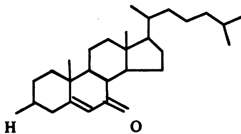
7-Ketocholesterol
