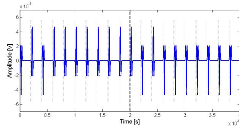
Fig. 4: Direct Sequence UWB Signal Simulation
