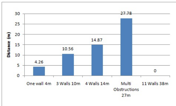
Fig. 11: Ranging Results of Hard-NLOS Area
