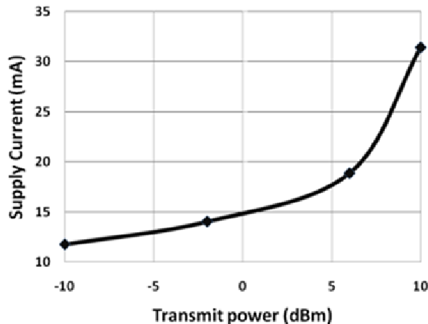
Figure 5. Relationship between wireless sensor current consumption and transmit power under a 50Ω load condition.
