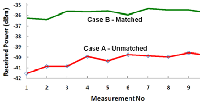
Figure 4. Measured received power before and after antenna tuning
