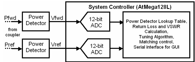
Fig. 6 Power detectors and system controller
