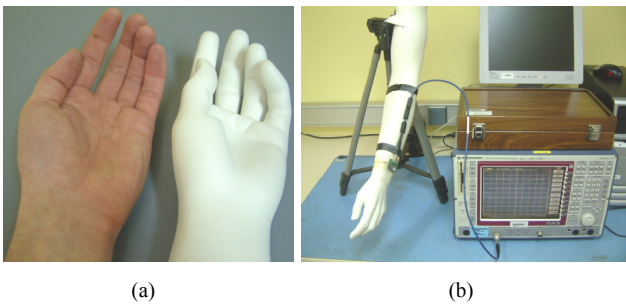
Fig. 3 (a) Human and phantom hand/wrist comparison, (b) VNA test setup
