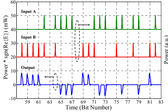
Fig. 2. The all-optical gate RZ-OOK inputs and RZ-DB output. \text{Re}\{E\} is the real part of the output electric field, and E has been rotated in the complex plane so as to be aligned with the real axis.
