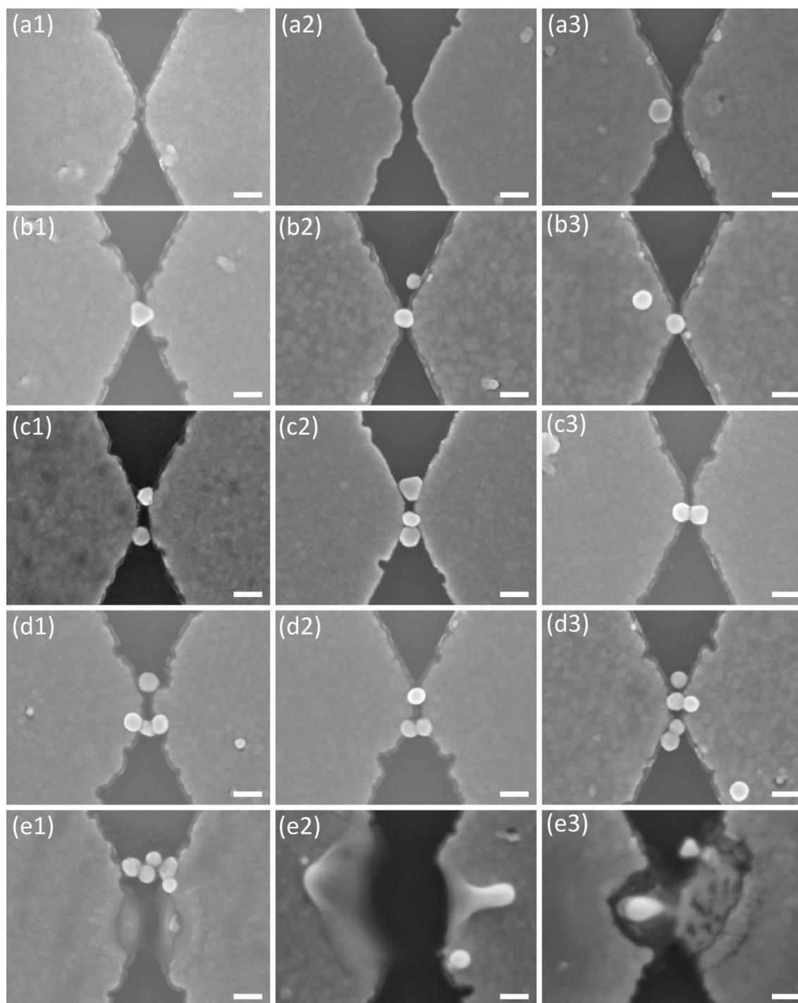
Figure 3.7. Compilation of Scanning Electron Microscopy images of typical nanocrystal assemblies. An overview of typical devices imaged by Scanning Electron Microscopy is presented. The scale bar is 100 nm in all images. Panels (a1-a3) show nano-scale gaps left empty after trapping (~25% of the cases). Panels (b1-b3) show the case of single particles trapped. Panels (c1-c3) show parallel or series assemblies. Together, panels (b) and (c) account for most trapping cases. Panels (d1-d3) present more complex nanocrystal assemblies (with both parallel and series nanocrystal bridging). Panels (e1-e3) show damage caused to the nanoscale gap during measurement for which a large bias was applied, |V_{ds}| > 0.5 V. Other damage patterns (not shown here) may be observed at the scale of a few micrometres as opposed to a few nanometres resulting from an ESD failure.
