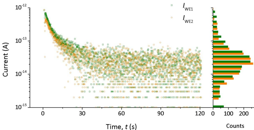
Figure 4.7. Minimising the ambient background electrical currents, \sim 30 fA is currently demonstrated in best conditions (in this test both spring-loaded probes contacting an empty nanoscale electrode gap were jointly biased under 0.5 V, current range reading was set to 100 pA with a resolution of 1 fA, 1 sample taken per measurement point: 1 measurement every \sim 20 ms).
