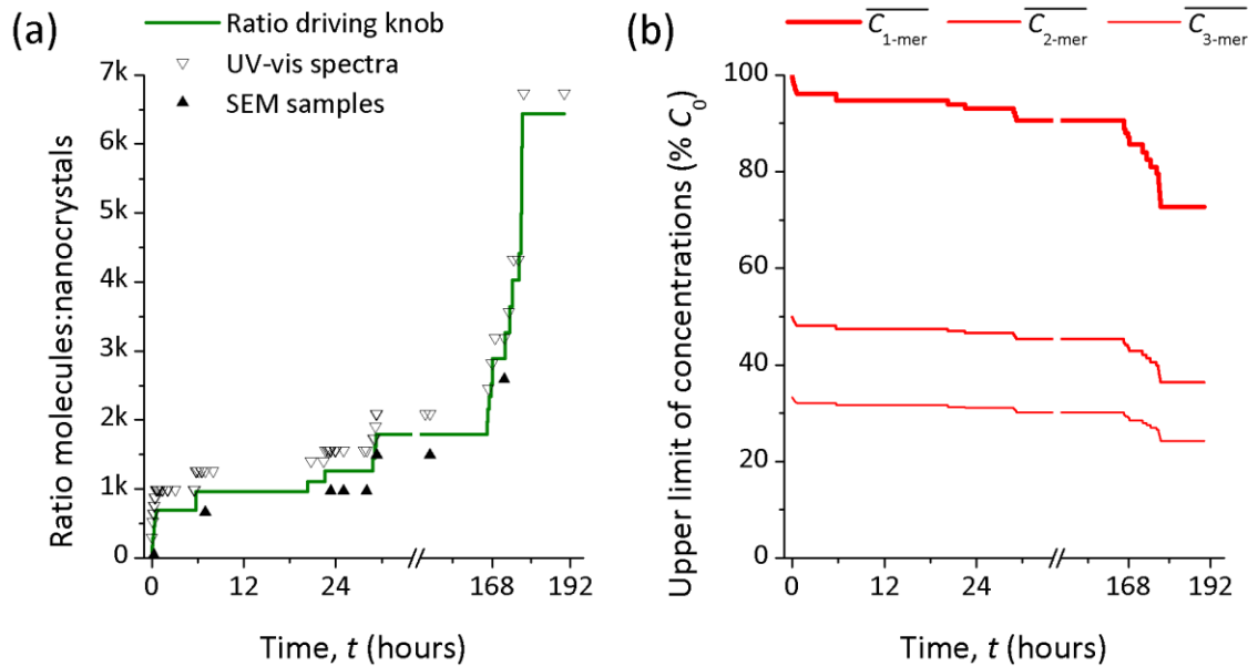
Figure 2.7. Design of experiment: a, the driving knob of the experiments: the molecule:nanocrystal ratio is plotted, open triangles show the times at which UV-vis absorption spectra were taken, filled triangles are for SEM samples; b, due to the addition of aliquots of linker molecules, nanostructures are diluted, the upper limit of concentrations are presented for 1-mers, 2-mers and 3-mers entities.
