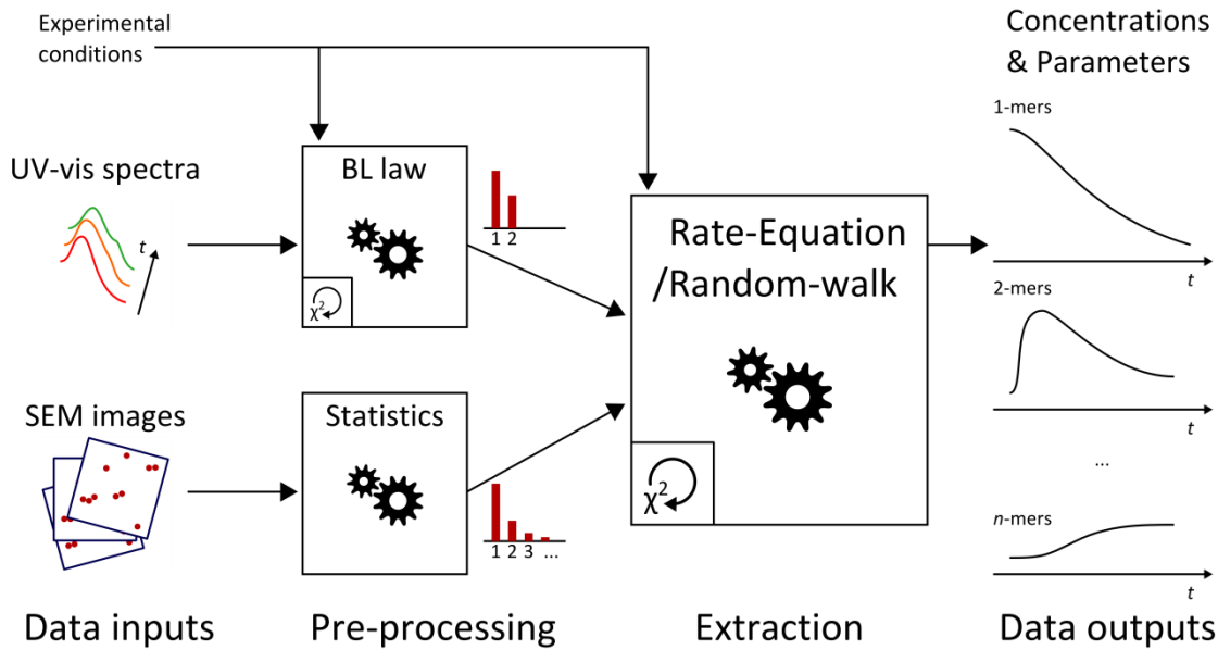
Figure 2.2 Simulation work-flow: UV-visible absorption spectra are processed using the Beer-Lambert law to obtain 1-mers and 2-mers concentrations, SEM images are analysed manually for counting the numbers of different n -mers present on the sample surface. The rate-equation model processes these data further to determine the evolution of the population of n -mers over time.
