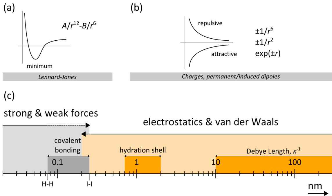
Figure 1.12. Schematic of pair potential and length scale: a, The shape of a typical Lennard-Jones is shown; b, interactions between charges, permanent/induced dipoles can give rise to repulsive or attractive potentials; c, domain of forces against the length-scale.
