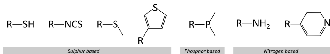
Figure 1.3. Variety of chemical anchor groups used in the field of research on molecular electronics ( \text{R} , stands for the main structure of the molecule), respectively: thiol, isothiocyanate, methyl sulphide, thiophene, dimethyl phosphine, amine and pyridine.
