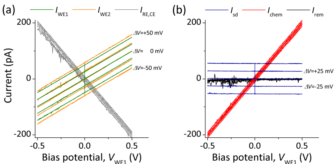
Figure 4.10. Example of artificial electrolytic gating on an assembly of a network of resistors: Z_{DUT} = 1 \text{ G}\Omega , Z_{SOL-WE1} = 5 \text{ G}\Omega , Z_{SOL-WE2} = 5 \text{ G}\Omega . (a) The bias is swept simultaneously on WE1 and WE2 with an offset potential between the two electrodes ( \Delta V ) that is sequentially increased from -50 mV to +50 mV by steps of 25 mV. (b) The transforms on currents show the source-drain conductance is constant, I_{sd} = (-I_{WE1} + I_{WE2})/2 (simple resistor: Z_{DUT} = 1 \text{ G}\Omega ), but the leakage current, I_{chem} = I_{WE1} + I_{WE2} , is not negligible and even dominates above \pm 0.2 \text{ V} . The remainder current is given by I_{rem} = I_{WE1} + I_{WE2} + I_{RE,CE} .
