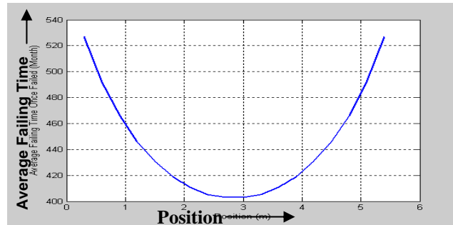
Figure 8. Time to Fail versus Position of Damage.
