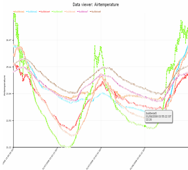
Figure 9. Full Graphical View of Temperature over 4 days
