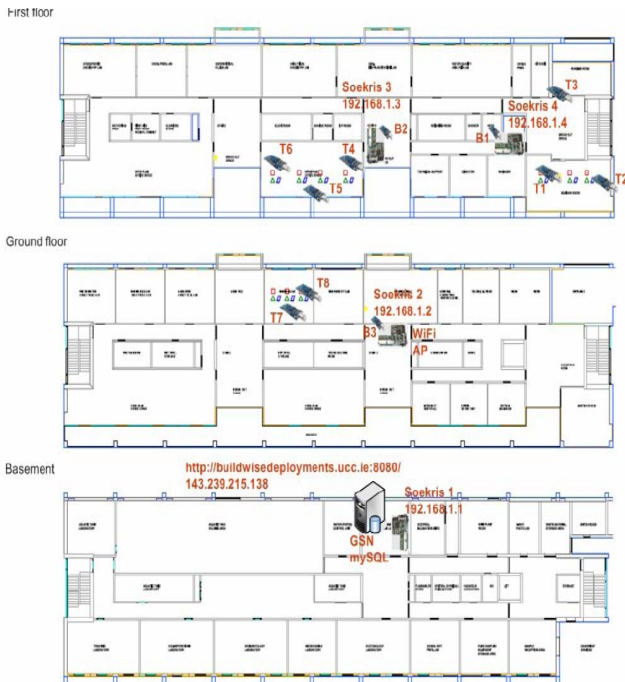
Figure 7. The established small scale WSN
