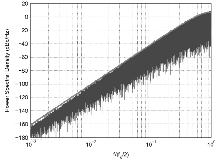
Fig. 29. Simulated PSD for N_3 when N = 20 , M = 14 , and L = 7 ; the input is 104 857. The smooth curve is \mathcal{L}_3(33) .
