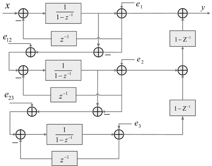
Fig. 8. Linearized model of the RC DDSM shown in Fig. 7.
