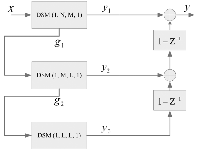
Fig. 7. RC MASH 111 DDSM using the notation of Fig. 6.
