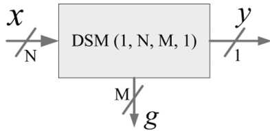
Fig. 6. Block diagram of the N -bit accumulator with an M -bit interstage quantizer.
