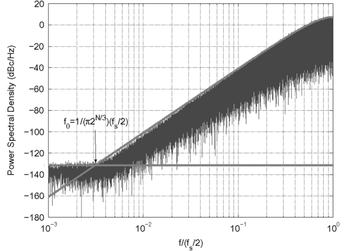
Fig. 30. Simulated PSD at the output of a zeroth-order dithered 20-bit MASH 111 DDSM; the input is 104 857. The dc term has been removed. The solid curves are \mathcal{L}_3 and \mathcal{L}_{nf_0} .
