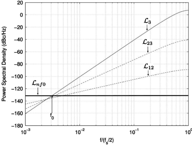
Fig. 25. Masking \mathcal{L}_{12} and \mathcal{L}_{23} below \mathcal{L}_3 at f_0 .
