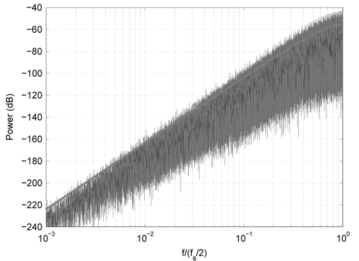
Fig. 3. Simulated power spectrum of a 20-bit third order DDSM; the input is 104 857. The smooth curve shows the ideal behavior of the 20-bit third-order DDSM, assuming that the quantization noise is white.
