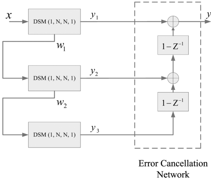
Fig. 5. Block diagram of a MASH 111 DDSM using the accumulator notation of Fig. 4.
