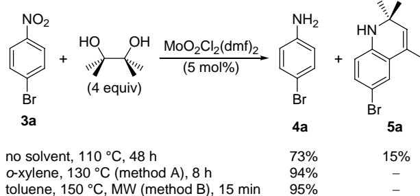
Scheme 2. Reduction of 4-bromonitrobenzene 3a using pinacol as deoxygenating agent.
