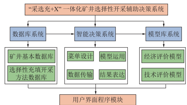
图 10 “采选充+X”一体化矿井辅助决策系统基本框架 [28] Fig.10 Basic block diagram of integrated mine auxiliary decision-making system of “mining, dressing and charging +X” [28]
