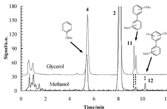
Fig. 3 HPLC traces of irradiated 4-chloroanisole ( 2 ) in methanol (bottom) and in a glycerol/methanol (4:1) mixture (top), under air, detected at 275 nm (initial concentration of 2 : 1 \times 10^{-2} M). Products 4 , 11 and 12 are anisole, dimethoxybiphenyls and chlorodimethoxybiphenyls, respectively.
