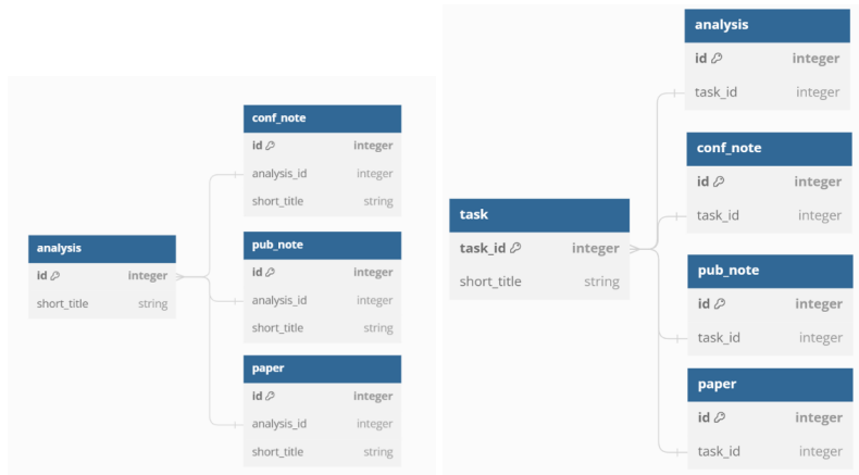
Figure 2. Model of denormalized schema. Figure 3. Model of the refactored normalized schema.
