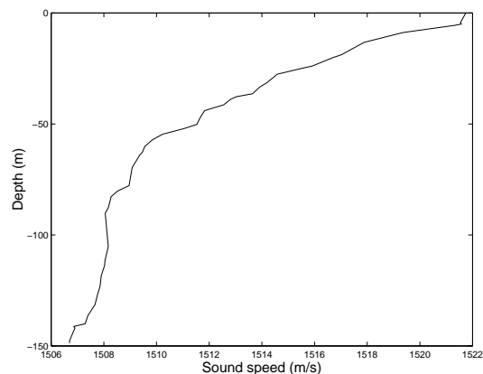
Fig. 3. Sound speed profile from XBT 48 (14:03).
