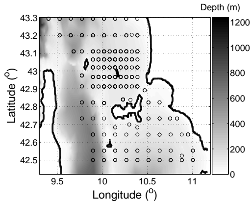
Fig. 4. Location of the CTD casts in the MREA'03 sea trial (circles) and bathymetric-range-independent transect considered in the simulations, centered on \approx (10.2^\circ, 43^\circ) (longitude,latitude).
