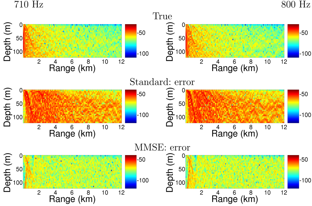
Fig. 11. True acoustic field and acoustic prediction errors obtained for JD 164.9, for the standard and MMSE predictors, at 710 and 800 Hz. The true field is represented as 20 \log_{10} |\mathbf{u}(r, z, f)| , while the error fields are represented as 20 \log_{10} |\mathbf{u}(r, z, f) - \mathbf{u}_{EST}(r, z, f)| .
