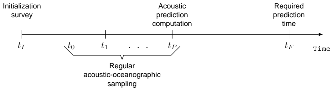
Fig. 2. Acoustic prediction time line. After the initialization of the oceanographic model at t_I , acoustic and oceanographic samples of the oceanic area of interest are taken on a regular basis, and the oceanographic model is run for the area, giving forecasts for t_0, t_1, \dots, t_P (present time) and t_F (required acoustic prediction time). All the acoustic-oceanographic information is combined, to predict the acoustics at t_F .
