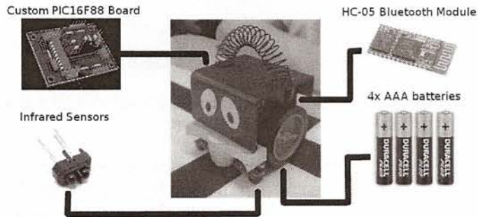
Fig. 2. Infante robot and its electronic parts
