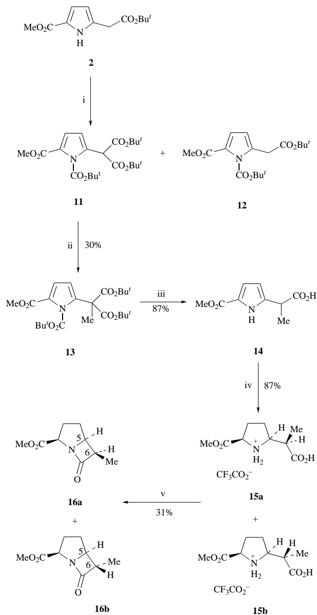
Scheme 4 Reagents and conditions: i , (\text{Bu}^t\text{O}_2\text{C})_2\text{O} , DMAP, room temp.; ii , KHMDS then MeI, -78^\circ\text{C} ; iii , TFA, room temp.; iv , \text{H}_2 (13.5 atm), Rh– \text{Al}_2\text{O}_3 , TFA, room temp.; v , 6 , \text{NEt}_3 , MeCN, 80^\circ\text{C}
