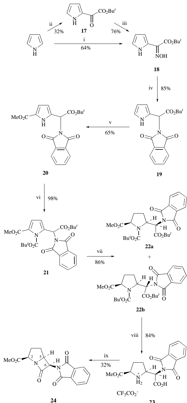
Scheme 5 Reagents and conditions: i , 25a , \text{Na}_2\text{CO}_3 , room temp.; ii , (\text{COCl})_2 , pyridine, -78^\circ\text{C} then \text{Bu}^t\text{OH} ; iii , \text{HONH}_3^+\text{Cl}^- , pyridine, 80^\circ\text{C} ; iv , Al–Hg then N -ethoxycarbonylphthalimide, \text{NEt}_3 , room temp.; v , (\text{Cl}_3\text{CO})_2\text{CO} , 110^\circ\text{C} , then MeOH, room temp.; vi , (\text{Bu}^t\text{O}_2\text{C})_2\text{O} , DMAP, room temp.; vii , \text{H}_2 (13.5 atm), Pt–C, room temp.; viii , TFA, room temp.; ix , 6 , \text{NEt}_3 , MeCN, 80^\circ\text{C}
