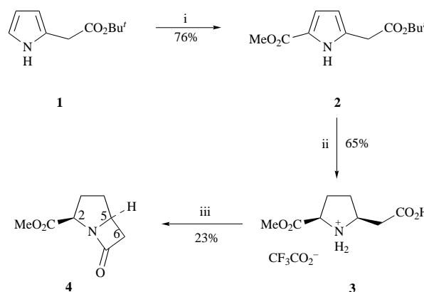
Scheme 2 Reagents and conditions: i, (CCl 3 CO) 2 CO, 110 °C, then MeOH, room temp.; ii, H 2 (13.5 atm), Rh–Al 2 O 3 , TFA, room temp.; iii, 6 , NEt 3 , MeCN, 80 °C
