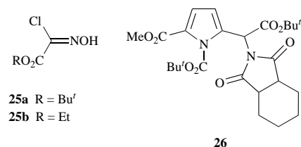
Scheme 5 Reagents and conditions: i , 25a , \text{Na}_2\text{CO}_3 , room temp.; ii , (\text{COCl})_2 , pyridine, -78^\circ\text{C} then \text{Bu}^t\text{OH} ; iii , \text{HONH}_3^+\text{Cl}^- , pyridine, 80^\circ\text{C} ; iv , Al–Hg then N -ethoxycarbonylphthalimide, \text{NEt}_3 , room temp.; v , (\text{Cl}_3\text{CO})_2\text{CO} , 110^\circ\text{C} , then MeOH, room temp.; vi , (\text{Bu}^t\text{O}_2\text{C})_2\text{O} , DMAP, room temp.; vii , \text{H}_2 (13.5 atm), Pt–C, room temp.; viii , TFA, room temp.; ix , 6 , \text{NEt}_3 , MeCN, 80^\circ\text{C}
