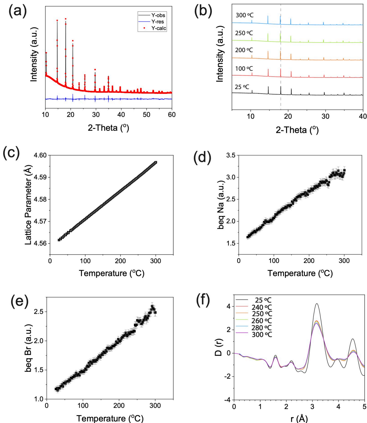
Figure 2. (a) Rietveld refinement of the room temperature synchrotron X-ray diffractograms of synthesised \text{Na}_3\text{OBr} with an X-ray wavelength of 0.825 318 Å. The black line is the experimental data, the red line is the fit, and blue line is the difference between them. (b) Variable temperature experiment. Sequential Rietveld refinements were performed on the variable temperature data, and the changes in (c) lattice parameter, (d) thermal parameter of Na ( b_{\text{eq}} Na), and (e) thermal parameter of Br ( b_{\text{eq}} Br) of \text{Na}_3\text{OBr} are plotted as a function of temperature. These show thermal expansion with no presence of crystalline deviation. (f) Differential correlation function D(r) calculated from experimental X-ray total structure factor F(Q) . Measurement was done with an X-ray wavelength of 0.161 669 Å.
