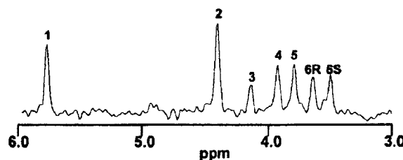
Figure 3. ^2\text{H} NMR spectrum of MAG prepared from a single plasma glucose blood sample of subject 4. The number above each signal represents its position in the glucose skeleton. The spectrum represents 53 850 free-induction decays for a total collection time of ~18 h
