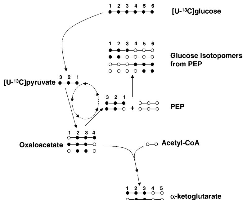
Figure 1. Fate of the ^{13}\text{C} of infused [\text{U}-^{13}\text{C}] glucose. Glycolysis in peripheral tissues generates [\text{U}-^{13}\text{C}] pyruvate and its equivalents. These are transported to liver and enter the hepatic Krebs cycle, principally as anaplerotic carbons via pyruvate carboxylase. Following carboxylation of [\text{U}-^{13}\text{C}] pyruvate, the initial [2,3,4-^{13}\text{C}_3] OAA product undergoes rapid exchange with malate and fumarate, resulting in \sim 50\% conversion to [1,2,3-^{13}\text{C}_3] OAA. Both isotopomers can be converted to [2,3-^{13}\text{C}_2] OAA as a result of the de-carboxylation and re-carboxylation reactions of pyruvate recycling (dotted arrows) coupled with \text{OAA} \leftrightarrow \text{MAL} \leftrightarrow \text{FUM} exchange. 19 Gluconeogenic outflow generates [\text{U}-^{13}\text{C}] and [2,3-^{13}\text{C}_2] PEP and the corresponding [1,2,3-^{13}\text{C}_3] - and [1,2-^{13}\text{C}_2] glucose isotopomers. These account for the majority ( \sim 85\% ) of glucose ^{13}\text{C} -enrichment derived from gluconeogenesis of [\text{U}-^{13}\text{C}] pyruvate. 29,30 The corresponding \alpha -ketoglutarate isotopomers generated from condensation of the OAA isotopomers with unlabeled acetyl-CoA are also shown
