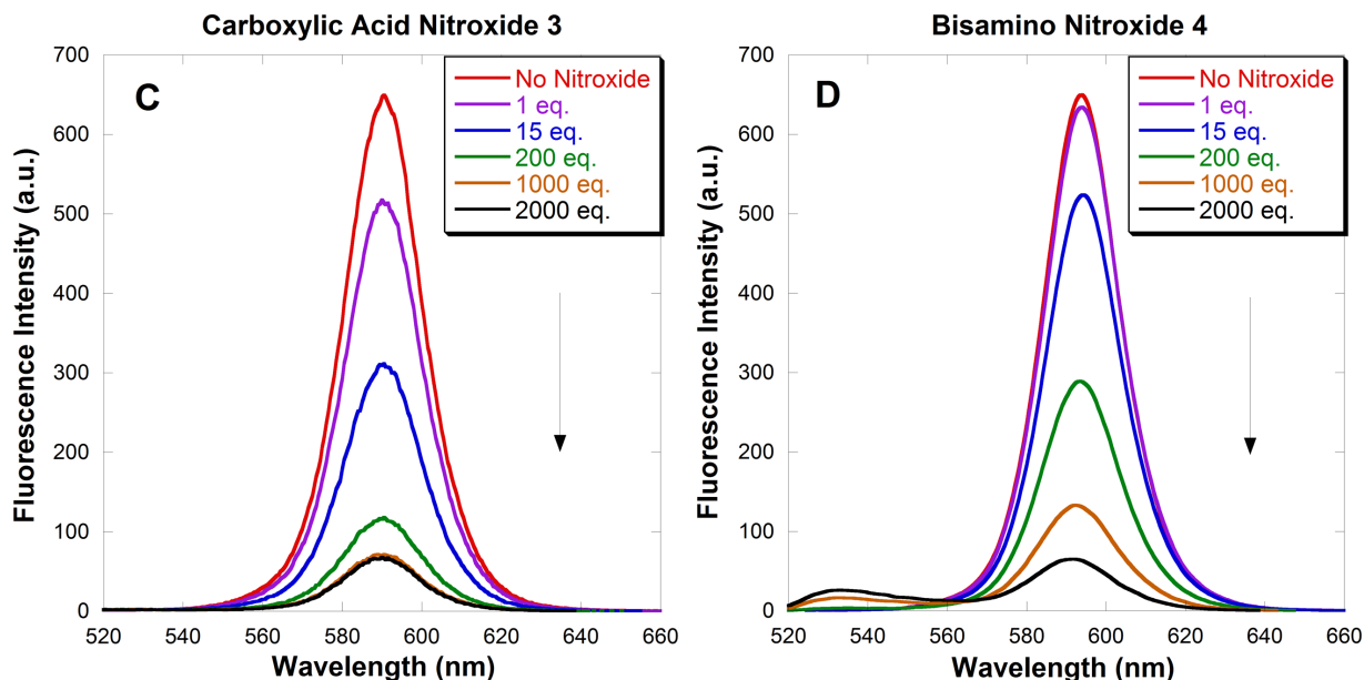
Figure 9A-D. Fluorescence emission spectra ( \lambda_{\text{ex}} = 390 \text{ nm} ) of toluene solutions of 3.7 nm CdSe QDs ( 0.4 \mu\text{M} ) quenched by increasing amounts of added nitroxides 1-4 . Spectra were taken 60 seconds after addition of each aliquot.
