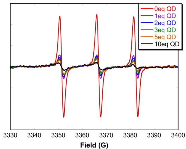
Figure 7. EPR spectra of carboxylic acid nitroxide 3 ( 0.5 \mu\text{M} ) in deaerated toluene with different concentrations of CdSe QDs. Spectra were taken after each aliquot was allowed to equilibrate for 24 hours.
