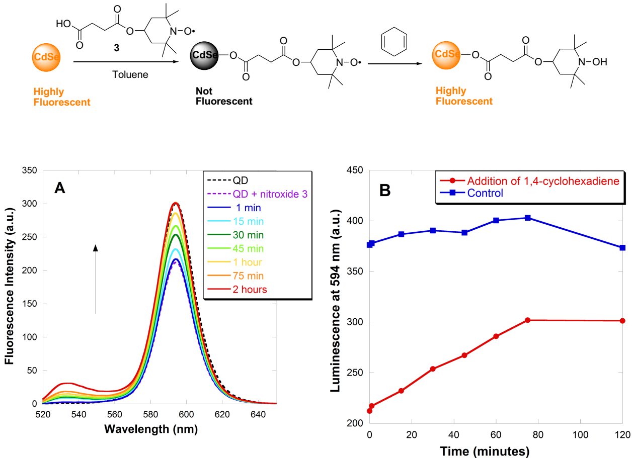
Figure 13. Fluorescence recovery of QD-carboxylic acid nitroxide 3 complex in toluene. Fluorescence emission spectra for an initial toluene suspension containing CdSe QDs (0.4 \mu\text{M} ) and carboxylic acid nitroxide 3 (1:17 moles of QD:nitroxide 3 ). At time = 0: 1,4-cyclohexadiene (100:1 moles of 1,4-cyclohexadiene:nitroxide 3 ) was added. (A) Emission spectra for excitation at 390 nm, and (B) emission intensity at the peak maximum of 594 nm.
