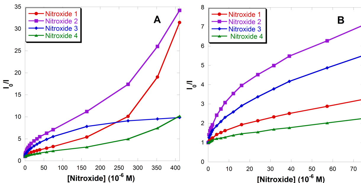
Figure 10. (A) Stern-Volmer plots of fluorescence quenching by nitroxides 1-4 at the emission maximum of 594 nm. (B) Enlargement for [\text{nitroxide}] < 77 \mu\text{M} ; I = observed fluorescence intensity, I_0 = fluorescence intensity with no nitroxide.
