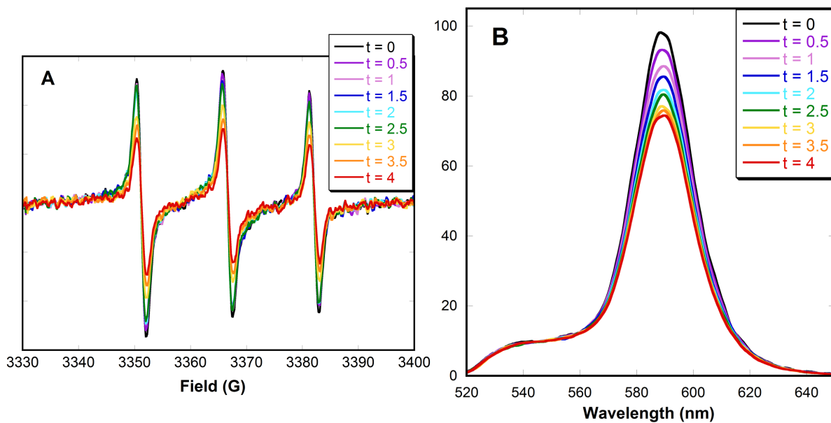
Figure 6. (A) EPR and (B) fluorescence spectra of carboxylic acid nitroxide 3 ( 0.5 \mu\text{M} ) with CdSe QDs ( 2 \mu\text{M} ) in deaerated toluene. Spectra were taken every 30 minutes for 4 hours.
