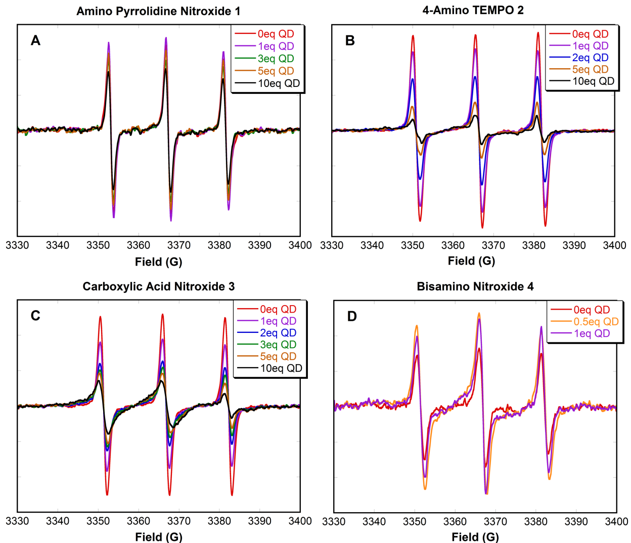
Figure 2A-D. EPR spectra of nitroxides 1-4 ( 0.5 \mu\text{M} ) in deaerated toluene upon successive addition of a solution of 3.7 \text{ nm} CdSe QDs. (Note: eq = equivalents)
