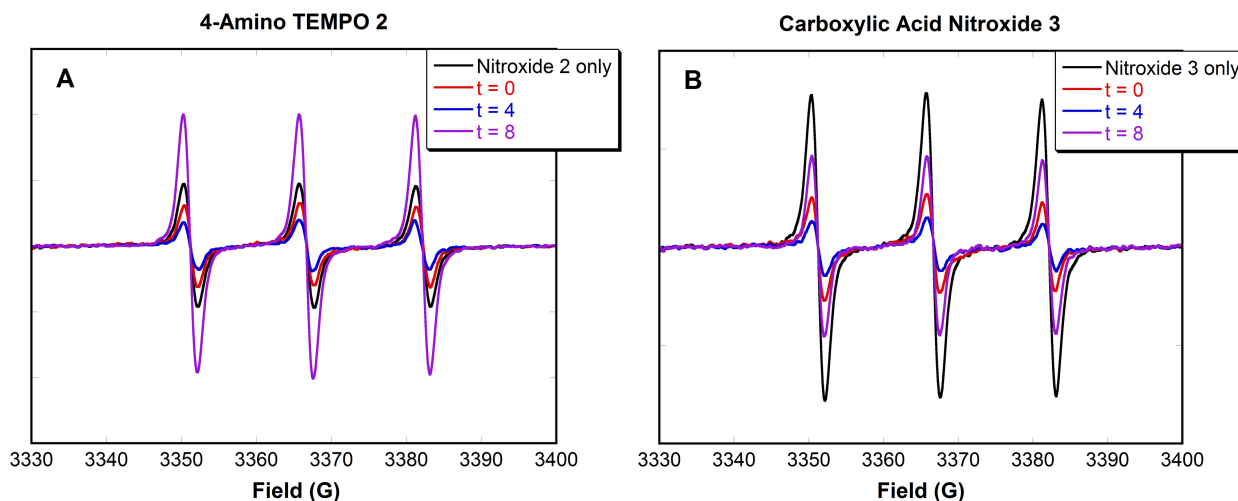
Figure 4. EPR spectra of a mixture of (A) 4-amino TEMPO 2 and (B) carboxylic acid nitroxide 3 ( 0.5 \mu\text{M} ) with CdSe QDs ( 2 \mu\text{M} ) in deaerated toluene. Spectra were taken at t = 0 and 4 h. At t = 4 h, a large excess of their corresponding competitors ( 6 \times 10^5:1 moles of competitor:nitroxide) was added, and spectra were taken at t = 8 h.
