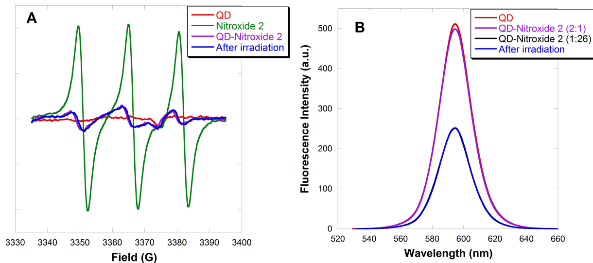
Figure 15. (A) EPR spectra and (B) fluorescence emission spectra of a benzene solution containing CdSe QDs (2 \mu\text{M} ), followed by addition of 4-amino TEMPO 2 (1 \mu\text{M} ) and
