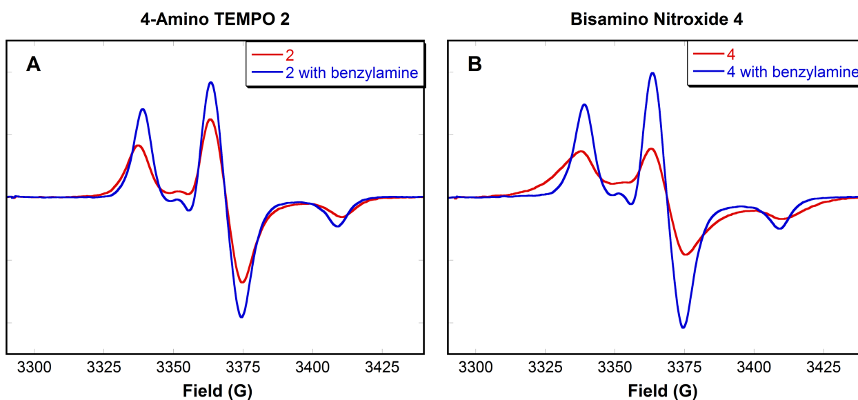
Figure 5A-B. EPR spectra of a mixture of 4-amino TEMPO 2 (50 \mu\text{M} ) or bisamino nitroxide 4 (200 \mu\text{M} ) with and without benzylamine ( 6 \times 10^5 :1 moles of benzylamine:nitroxide) in deaerated p -xylene. Spectra were recorded at 125 K.
