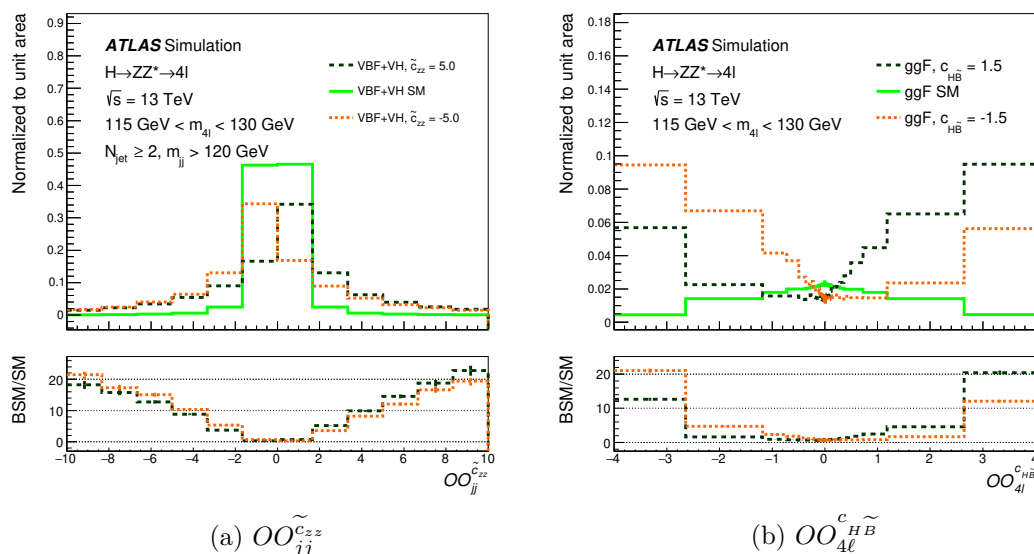
Figure 3. Expected distributions of (a) the OO_{jj}^{c_{zz}} observable for VBF-produced Higgs boson candidates combining VBF SR1 through SR4 for the SM and for BSM coupling parameter values of \tilde{c}_{zz} = \pm 5 , and (b) the OO_{4\ell}^{c_{HB}} observable for the decay of ggF produced Higgs boson candidates in the inclusive SR for the SM and for BSM coupling parameter values of c_{HB} = \pm 1.5 . (a) has 12 equal-size bins, and (b) has 48 equal population bins. In (b) the first and last bins extend up to \pm 40 , but the bin range is truncated to \pm 4 in the plot for clarity. The lower panels show the ratio of the BSM to the SM optimal-observable distributions.
