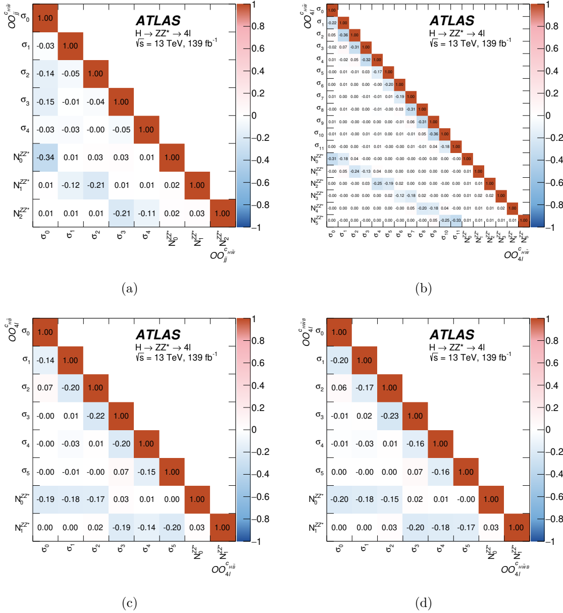
Figure 15. Correlation matrices between the measured differential fiducial cross-section and ZZ^* normalization bins for the (a) OO_{jj}^{c,H\tilde{W}} , (b) OO_{4l}^{c,H\tilde{W}} , (c) OO_{4l}^{c,H\tilde{B}} and (d) OO_{4l}^{c,H\tilde{W}B} optimal observables. The bin labeled \sigma_0 of (a) is not part of the OO_{jj}^{c,H\tilde{W}} differential distribution, but contains events with fewer than two selected jets with p_T > 30 GeV.
