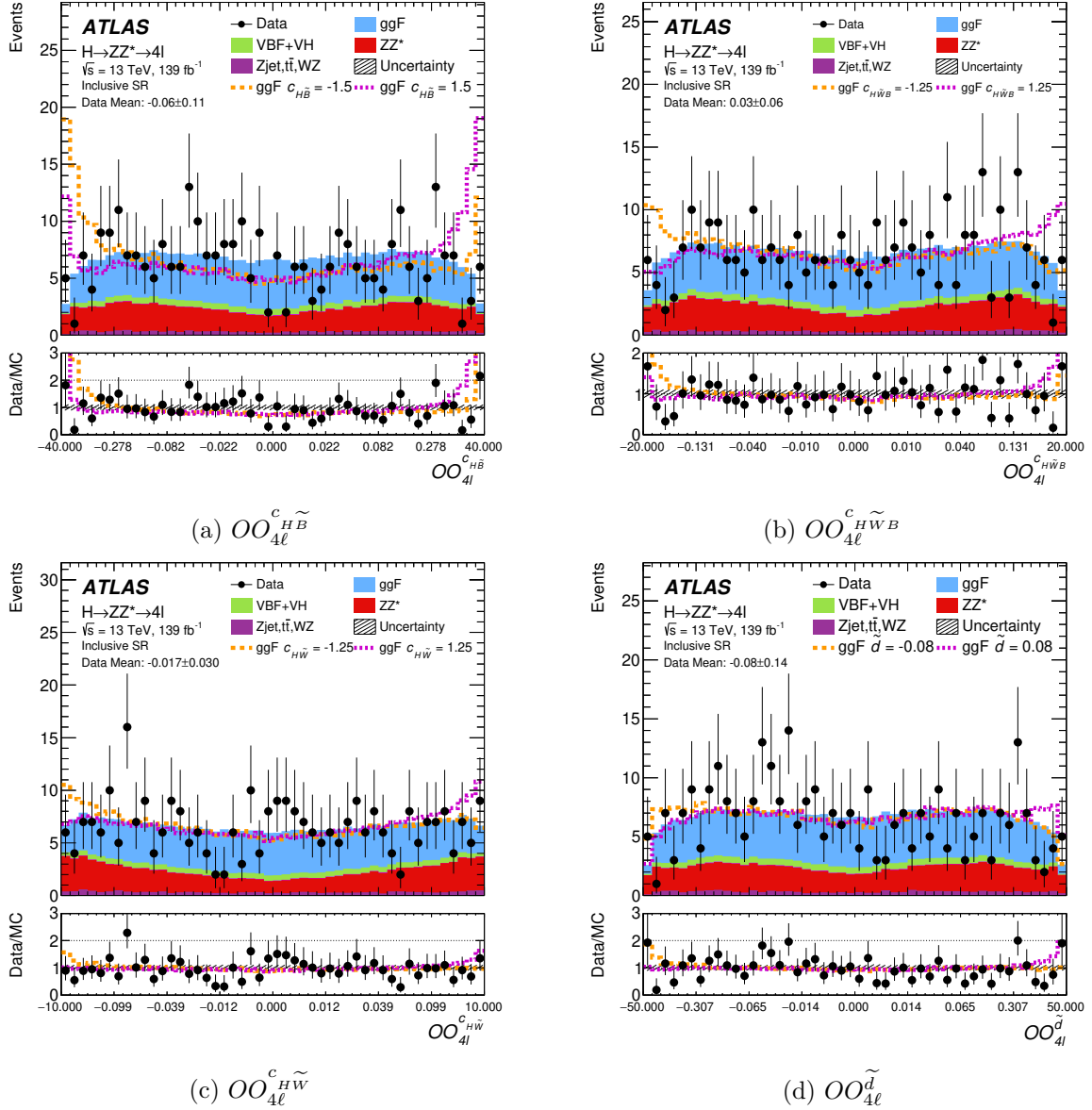
Figure 6. The observed and expected distributions for the decay level observables: (a) OO_{4l}^{c_{HB}} , (b) OO_{4l}^{c_{HWB}} , (c) OO_{4l}^{c_{HW}} and (d) OO_{4l}^{\tilde{d}} . The expected distribution for the ggF and VBF signals and the backgrounds from ZZ^* and reducible backgrounds are shown as a stacked histogram. Also shown are the expected distributions in presence of CP-odd contributions for (a) c_{HB} = \pm 1.5 , (b) c_{HWB} = \pm 1.25 , (c) c_{HW} = \pm 1.5 and (d) \tilde{d} = \pm 1.25 , assuming the signal event rate remains that of the SM. The bin size is variable, optimized for an approximately flat distribution for the SM combined with a positive and negative BSM scenario. There are no observed events that fall outside the optimal-observable distribution range, with rate expectations below 0.1%. The mean value of the optimal observable across the data events is given with its standard deviation. The lower panels show the ratio of data to expectation and the shaded band corresponds to the combined statistical and systematic uncertainties in the predictions.
