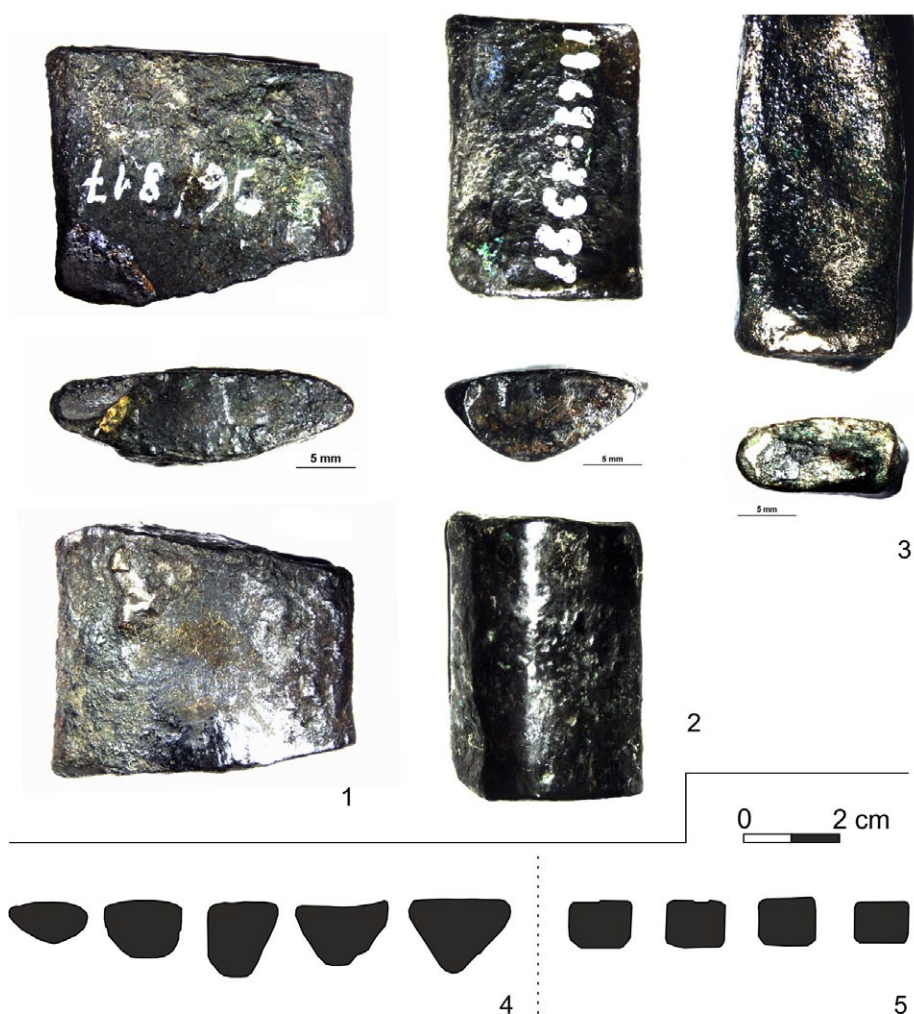
Fig. 3. 1-3: Selected fragments of cast ingots from Wicina (1: Wi_97_817, 2: Wi_69_2387, 3: Wi_69_2378). 4: Cross-sections of cast ingots from Wicina. 5: Cross-sections of cast-and-forged bronze ingots from the Bieszków hoard
