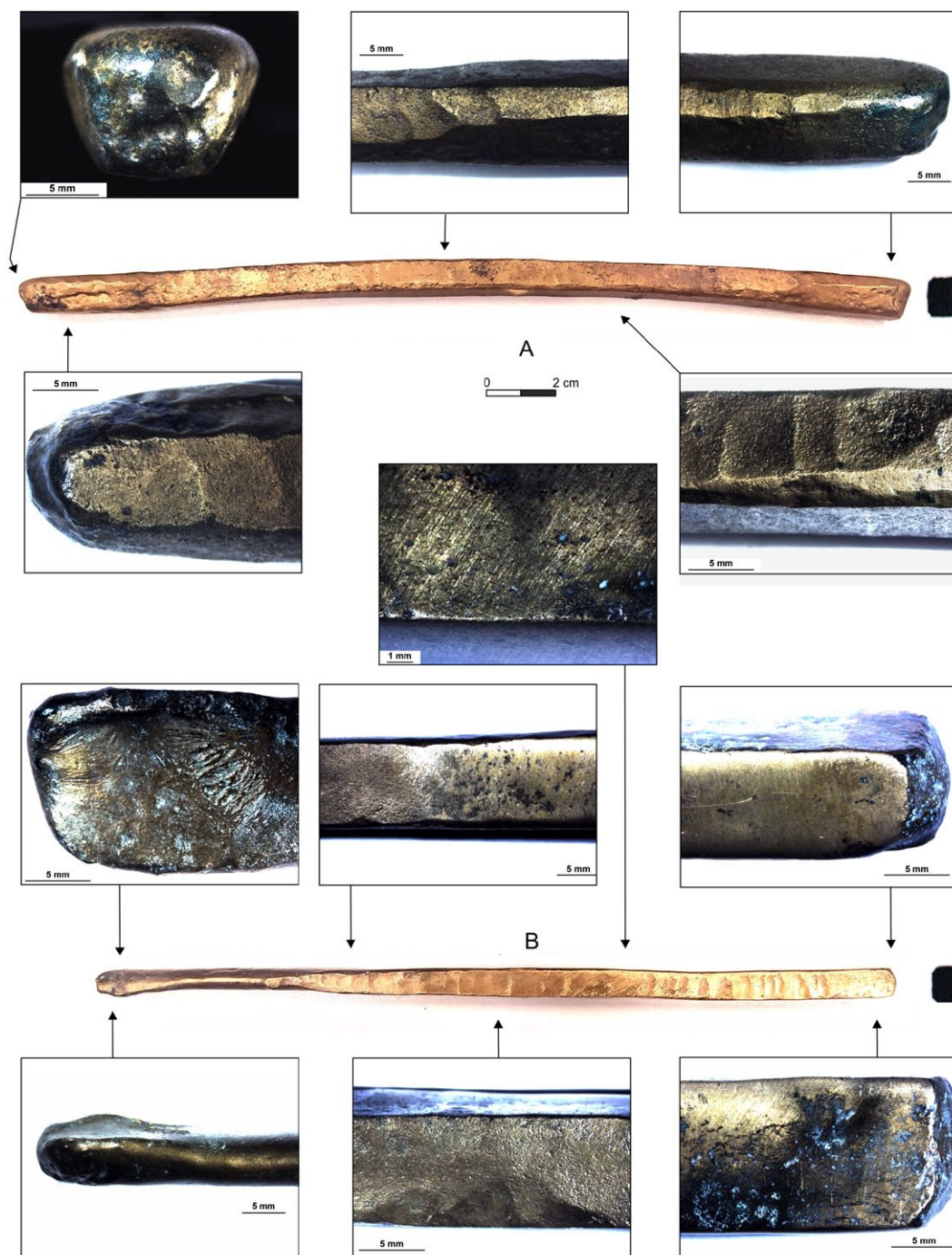
Fig. 4. Optical microscopy (OM) images of the cast-and-forged ingots from the Bieszków hoard (A: Bi_12_240, B: Bi_12_241). Different degrees of plastic processing are evident: in the case of Bi_12_240, forging of the top surface and edges; in the case of Bi_12_241, forging, modeling to rectangular section, and grinding of all planes, but limited to about two-thirds of the bar length
