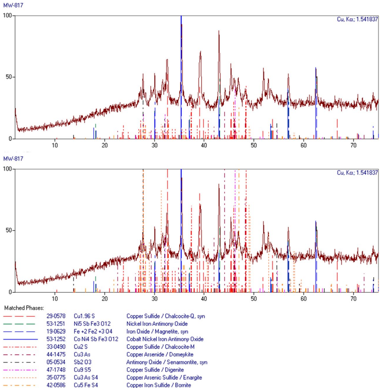
Fig. 13. X-ray diffraction data from powdered samples of the Wi_97_817 ingot, with the particle size on the order of 0.1 mm
