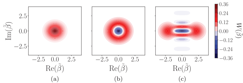
Fig. 7.3 Wigner functions of different states. (a) A vacuum state represented by a coherent state with |\alpha| = 0 . (b) Wigner function for a Fock state |n = 1\rangle . (c) Wigner function of a coherent state superposition |\alpha\rangle - |-\alpha\rangle , with |\alpha| = 1.5 .
