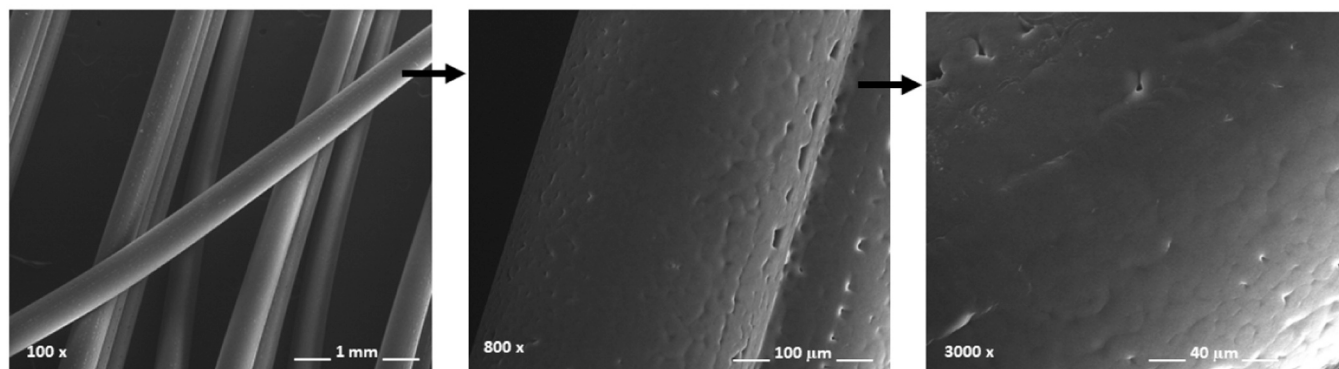
Fig. 1. SEM images of fibre meshes prepared by melt electrospinning using PCL with 0.05 % daunorubicin (D1) and 0.025 % daunorubicin (D2).
