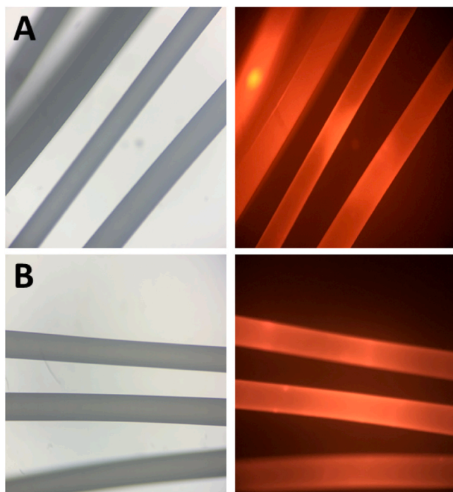
Fig. 2. Bright and fluorescence images taken by fluorescence microscopy for A: D1 meshes loaded with 0.05 % daurorubicin and, B: D2 meshes loaded with 0.025 % daurorubicin.
