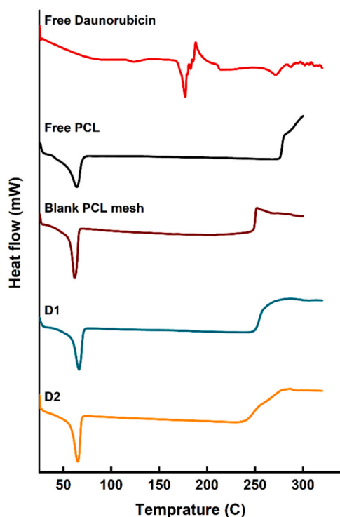
Fig. 4. DSC analysis of free PCL, free daunorubicin, and electrospun fiber meshes D1 and D2 loaded with varied percentages of daunorubicin.
