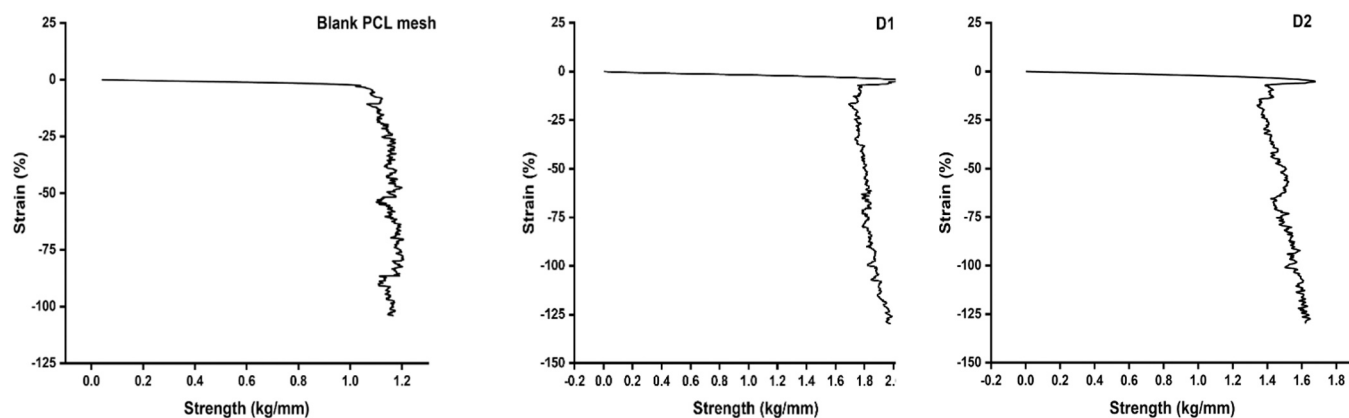
Fig. 8. The ultimate strength (kg/mm) vs the strain (%) when the meshes are stretched.
