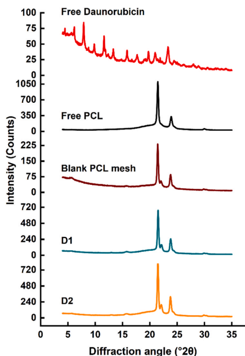
Fig. 6. XRD patterns of PCL pellets, free daurubicin, and electrospun fiber meshes as empty or loaded with various percentages of daurubicin.
