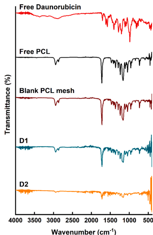
Fig. 5. FT-IR spectra of free daunorubicin hydrochloride, free PCL, empty meshes, and daunorubicin loaded meshes containing 0.05 % (D1) and 0.025 % (D2).
