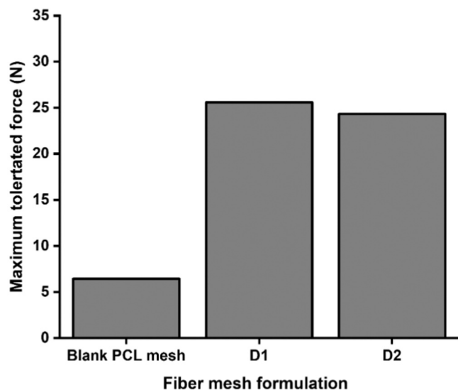
Fig. 7. The tensile strength of empty and drug loaded PCL meshes expressed as the maximum tolerated force ( n=3 ).
