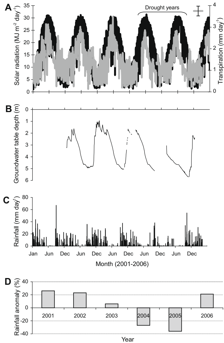
Fig. 1. Long-term evolution of (A) daily tree transpiration ( Quercus ilex , n = 4 ) per unit of crown projected area ( T_t , grey line) and solar radiation (black line) and (B) and (C) other environmental variables (B – groundwater table depth and C – rainfall), from 2001 to 2006. Rainfall anomaly to long-term annual average (669 mm, 1961–1990) is also represented (D). In (A) the error bar is the average standard error of tree transpiration.
