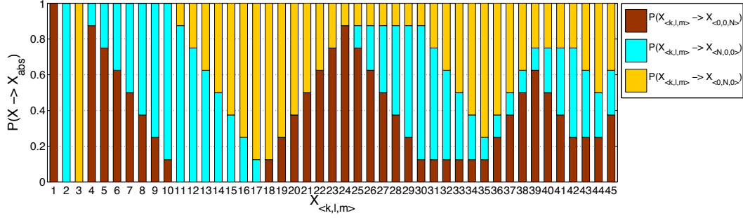
FIGURE 9. The probabilities of reaching the three absorbing states for all initial nodes X_{\langle k,l,m \rangle} . Notice that all three final states can be reached only from the inner nodes (numbers 25 to 45).
