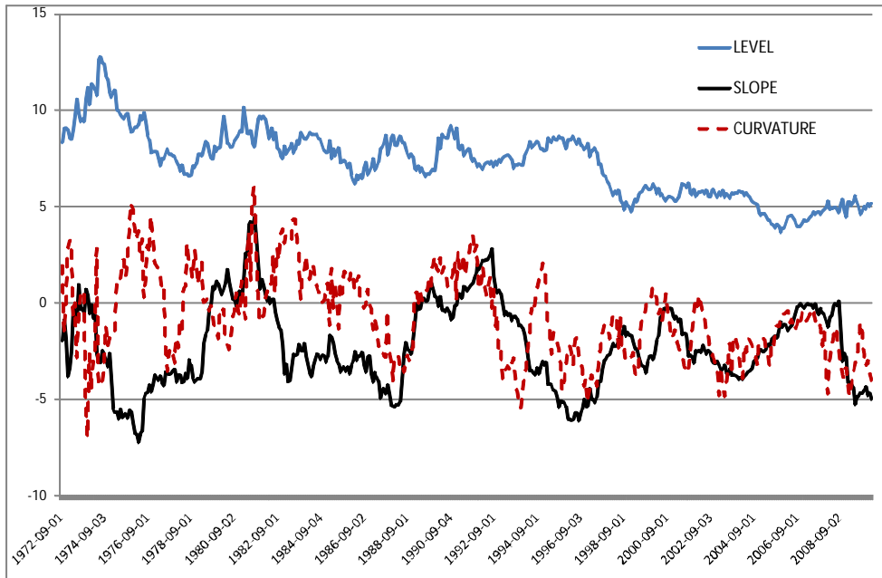
Figure 5. Estimates of L_t , S_t and C_t , Germany 1972:9-2010:3
