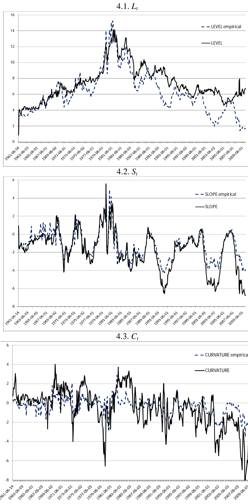
Figure 4. Estimates of L_t , S_t , C_t , and empirical proxy, U.S. 1961:6-2010:2
