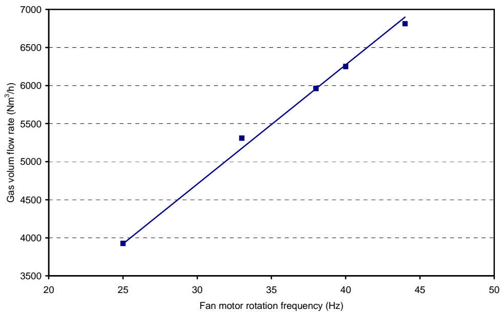
Figure 1. Relationship between the gas volume flow rate and the fan rotation frequency in the dryer stack.
