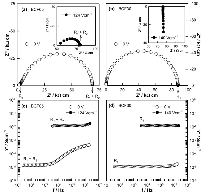
Figure 3. Impedance complex plane plots (a,b) and Y' spectroscopic plots (c,d) at \sim 30 °C before and after a voltage was applied.
