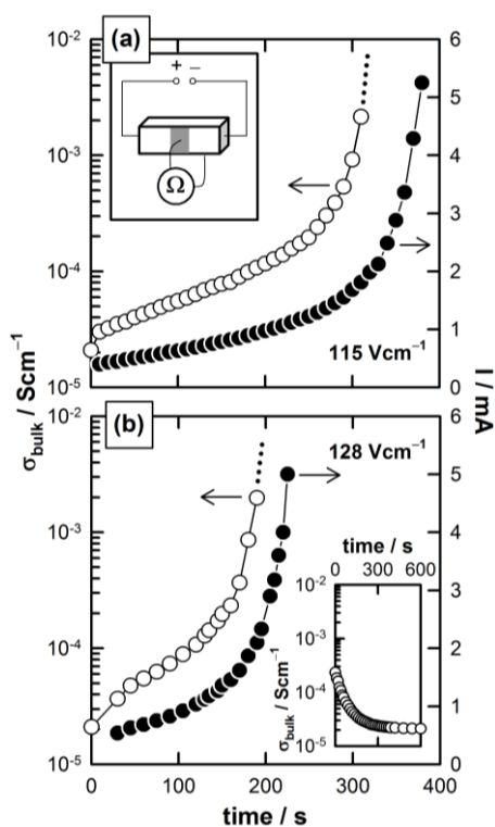
Figure 7. BCF30: dc conductivity and current perpendicular and parallel to the direction of the applied voltage, respectively, against time for several dc bias voltages at ~50 °C. Inset in (a): schematic setup for dc conductivity measurements perpendicular to the direction of the dc bias. Inset in (b): dc conductivity vs time on removal of the dc bias.
