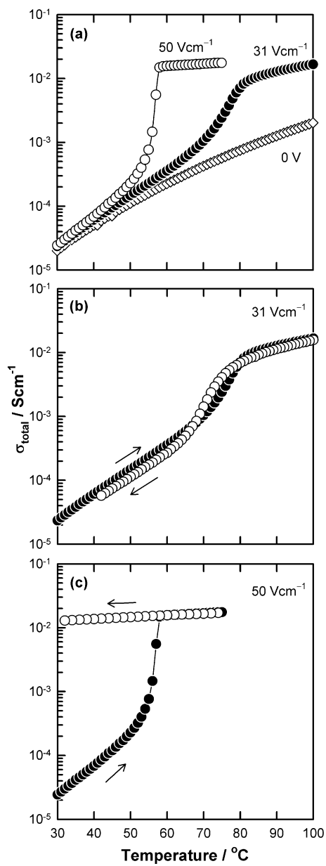
Figure 9. BCF05: total conductivity vs temperature after a range of voltages was applied.
