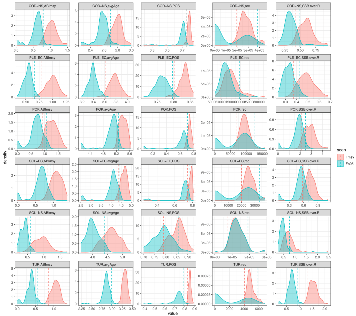
Figure 6.6.2 Distribution of the indicators ABImSY, avgAge, POS, R, SSB/R at F_{MSY} and F_{P0.5} , with the associated 5 th and 95 th percentile (dotted vertical lines), calculated for the stocks of COD-NS, PLE-EC, POK, SOL-EC, SOL-NS, TUR.
