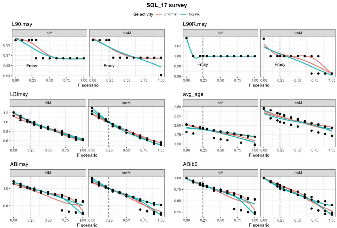
Figure 5.4.16 length based (L90.msy, L90R.msy, LBI.msy) and age based (avg_age, ABImSY and ABIB0) indicators calculated on length-based simulations for SOL_17 at F scenarios calculated on the population at sea sampled with survey selectivity. Dotted vertical line represent the F at msy estimated from the most updated stock assessment. Panels show the alternative natural mortality vectors used (high mortality hiM and low mortality lowM), solid lines show the trend when using alternative fishery selectivity (doublenormal in pink and logistic in blue).
