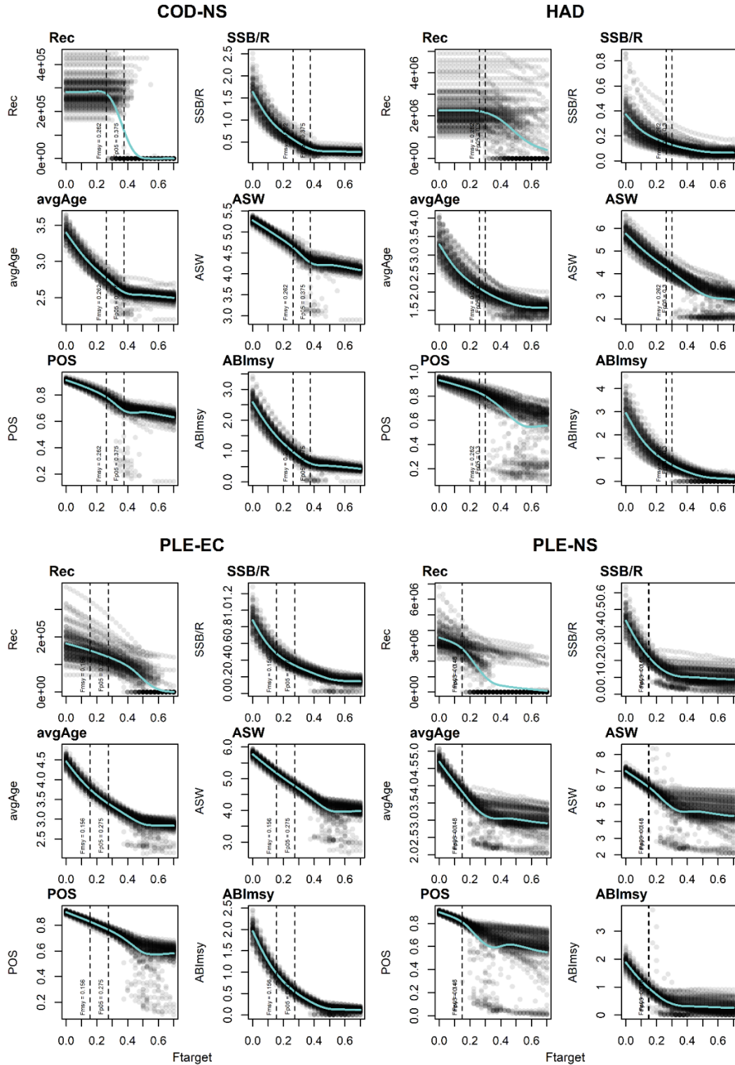
Figure 5.2.2.2: D3C3 indicators (Rec – Recruitment, SSB/R, ASA – average spawner age, ASW – average spawner weight, POS – proportion of old spawner and ABImSY) under different Ftargets for the stocks cod, haddock and plaice (North Sea and English Channel); overlaid are the estimated F_{msy} and F_{p05} reference points as dashed lines as well as a smoothing line (blue) for easier visualisation.
