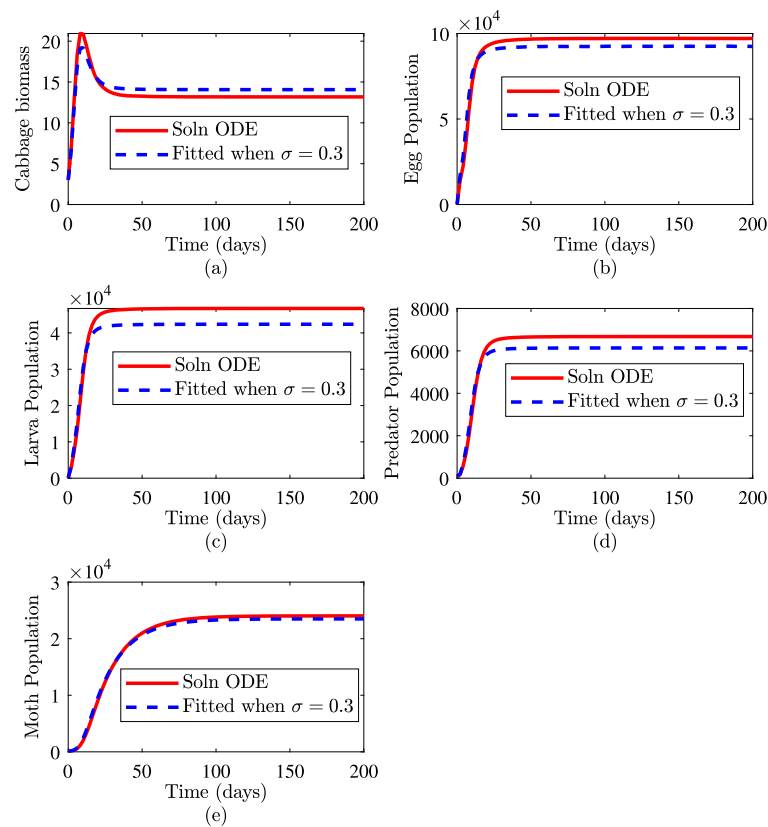
Fig. 12. Illustrates the ODE solution versus the fitted solution.
