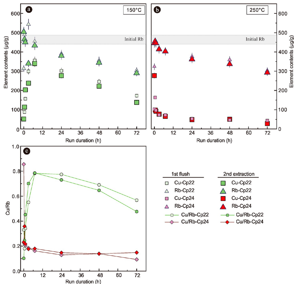
Figure 9. Variation of element contents of solutions as a function of time. (a) Run Cp22, 150 °C, 20 MPa, 72 h; (b) run Cp24, 250 °C, 20 MPa, 72 h. (c) The Cu/Rb ratio (in µg/g) of the 1st and 2nd solutions varies with time. Both experiments were loaded with Cu 2 O and 0.2 m HAC/KAc solutions.
