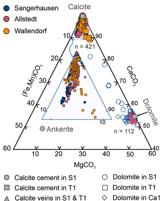
Fig. 7. Ternary diagram of \text{CaCO}_3\text{-(Fe,Mn)CO}_3\text{-MgCO}_3 (EPMA, mol%) showing endmember calcite and dolomite in samples from the Rotliegend sandstone (S1), Kupferschiefer (T1) and Zechstein Limestone (Ca1) in the Sangerhausen, Allstedt and Wallendorf drill cores.
