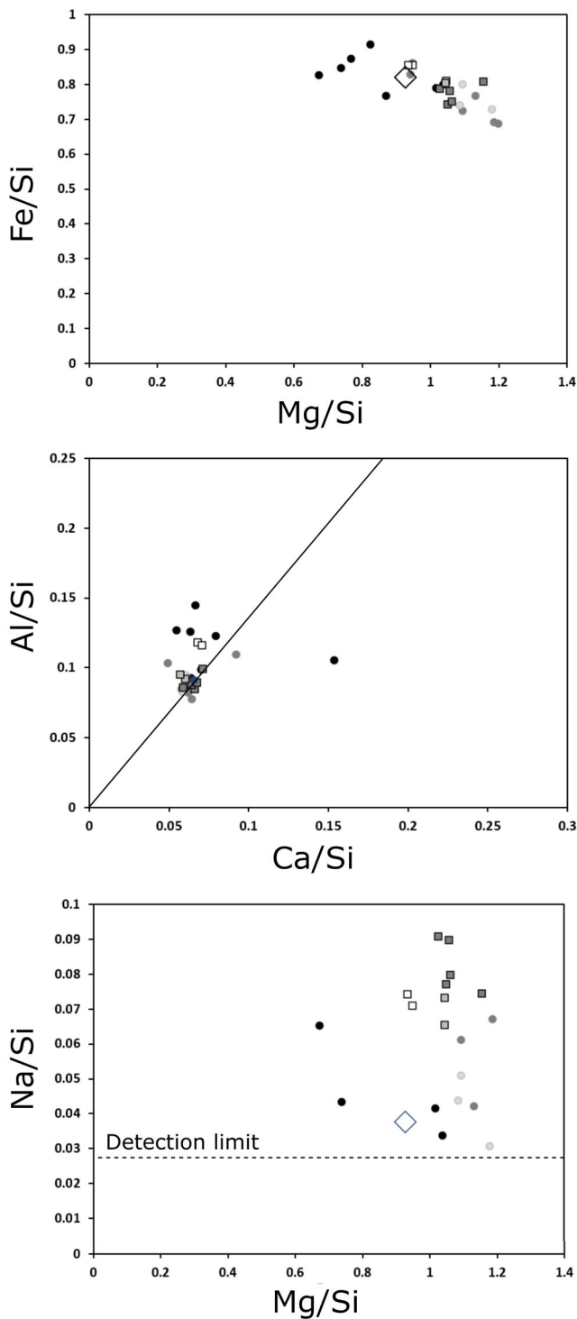
Fig. 9. Compositions of fusion crust of P30555 determined by area EDS analyses as atomic ratios. Symbols: outer melted crust—solid light gray circles, mid melted crust—medium gray circles, inner melted crust—solid black circles, silicate wart b—mid gray squares, silicate wart c—light gray squares, silicate wart d—white squares, bulk composition (King et al., 2022)—diamond. (Color figure can be viewed at wileyonlinelibrary.com )
