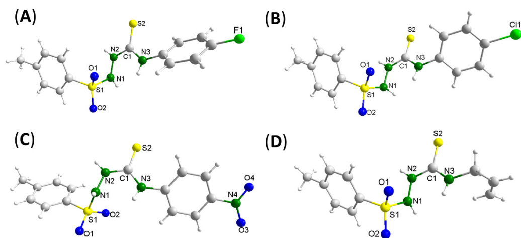
Figure 2. Molecular structures of the free ligands \text{HL3}^{\text{FPh}} (A), \text{HL4}^{\text{ClPh}} (B), \text{HL5}^{\text{NO}_2\text{Ph}} (C) and \text{HL6}^{\text{Al}} (D) obtained by single crystal X-ray diffraction.
