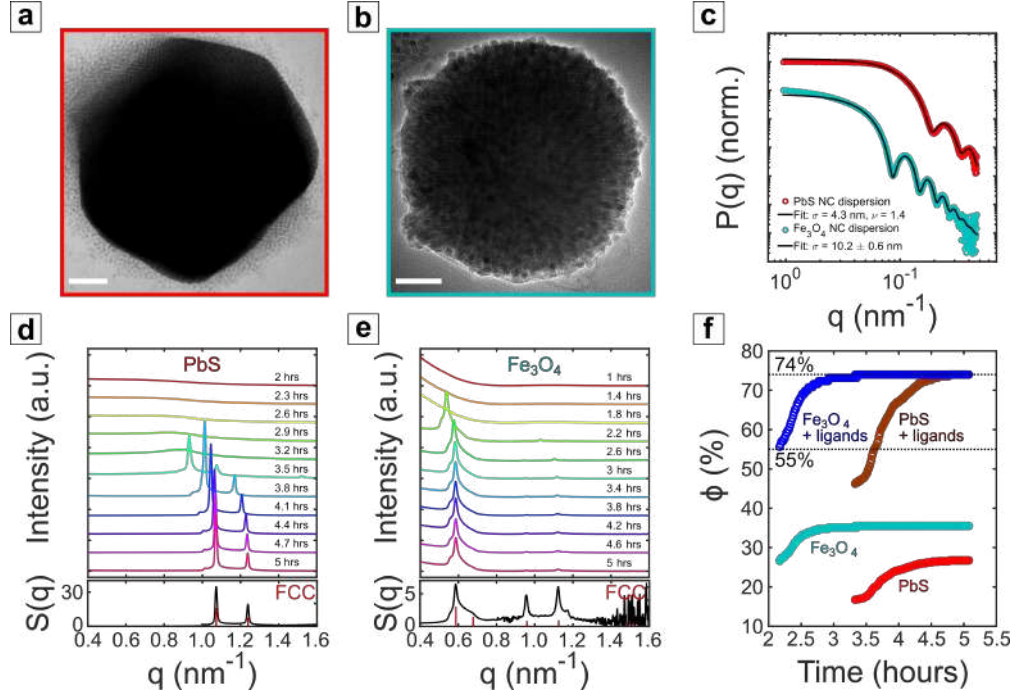
Figure 5: In situ observation of supercrystal formation. (a-b) Transmission electron micrographs of supercrystals of (a) PbS and (b) \text{Fe}_3\text{O}_4 NCs. Scale bars indicate 50 nm. (c) Experimental form factors (symbols) and fit (solid lines) of PbS and \text{Fe}_3\text{O}_4 NCs. (d-e) Azimuthally-averaged SAXS patterns of (d) PbS and (e) \text{Fe}_3\text{O}_4 NCs undergoing crystallization while dispersed within toluene droplets in 24g/L SDS in water at 70°C. Time stamps are indicated for each curve. The structure factor, S(q) , extracted from the last curve is shown at the bottom of each panel. Expected positions for FCC reflections are indicated by red ticks. (f) Kinetic evolution of the FCC volume fraction, \phi , relative to the inorganic core of NCs (lighter symbols) as well as to their hard sphere size (darker symbols). The dotted lines indicated the hard sphere melting transition, \phi \approx 55\% , and close packing, \phi \approx 74\% .
