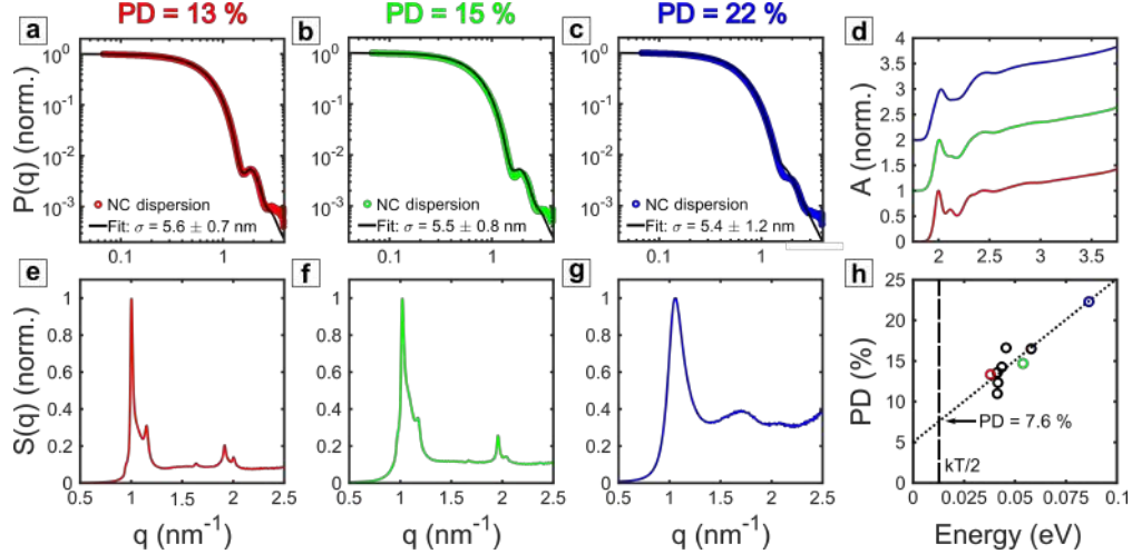
Figure 4: Influence of NC polydispersity on the final quality of supercrystals based on CdSe NCs. (a-c) Determination of NC polydispersities from measured form factors. 24 Experimental form factors (dots) and fits to spherical form factors (solid lines) of NCs of comparable mean diameters and increasing polydispersity: (a) \sigma = 5.6 \pm 0.7 \text{ nm} , (b) \sigma = 5.5 \pm 0.8 \text{ nm} , (c) \sigma = 5.4 \pm 1.2 \text{ nm} . (d) Absorption spectra measured from dispersions of NCs described in (a-c). (e-g) Structure factors measured from supercrystals consisting of NCs described in (a-c), respectively, dried at 20^\circ\text{C} from a cyclohexane emulsion stabilized by 6 \text{ g/L} SDS in water. (h) Dependence of the NC polydispersity, determined through SAXS, on the half-width at half-maximum (HWHM) of the lowest-energy excitonic transition, determined through spectrophotometry. Colored dots correspond to the samples described in (a-g). The dotted line indicates the linear fit: PD(\%) = 5.015 + 201.2 \times HWHM(eV) .
