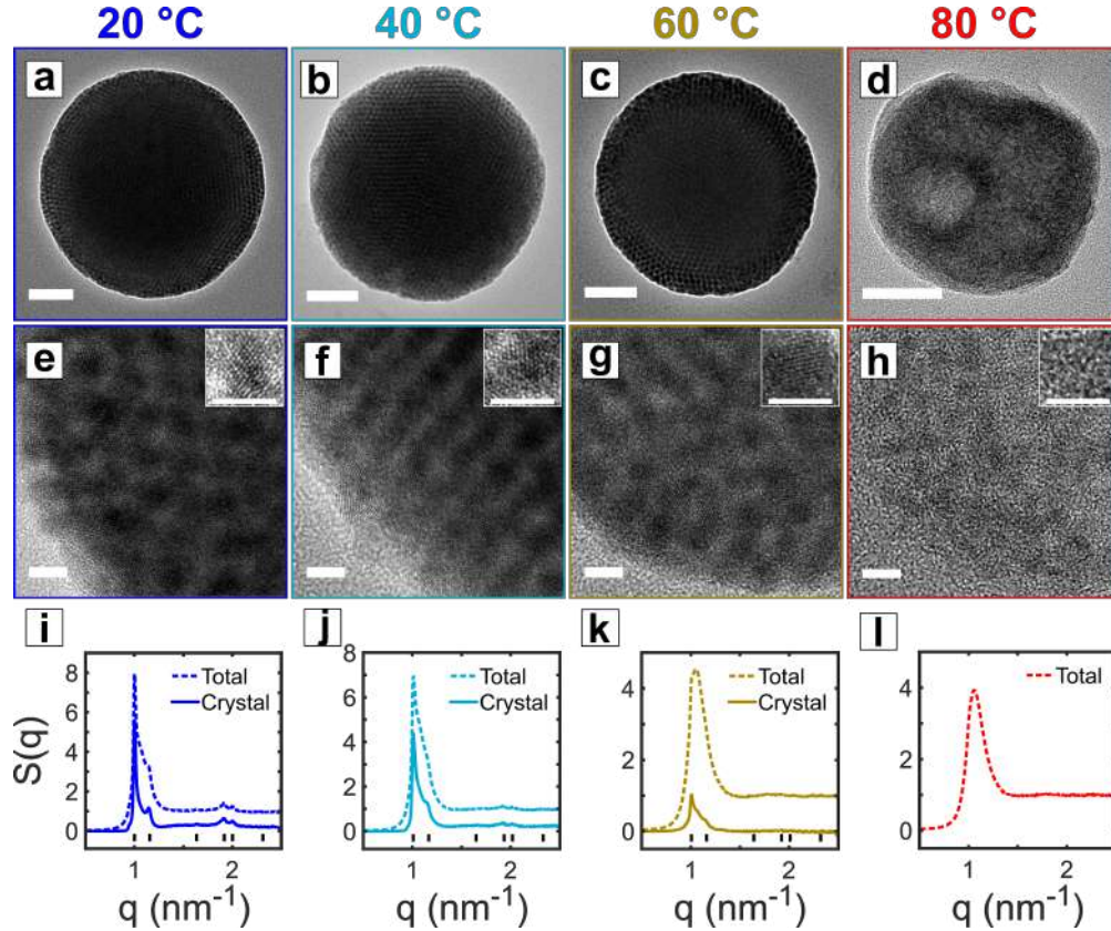
Figure 2: Influence of the evaporation rate on supercrystal quality. Intermediate (a-d), and high (e-h) resolution TEM micrographs of superstructures assembled from an emulsion dried at the indicated temperature. The dispersed phase consisted of a dispersion of \sigma = 5.6 \pm 0.7 \text{ nm} CdSe NCs in cyclohexane at an initial volume fraction of \phi \approx 0.09\% , while the continuous phase consisted of a solution of 6 \text{ g/L} SDS in water. The insets show zoomed-in view of a NC embedded in the superstructure. Scale bars indicate: 50 \text{ nm} (a-d), and 5 \text{ nm} (e-h). (i-l) Experimental structure factors of supercrystals dried at the indicated temperatures.
