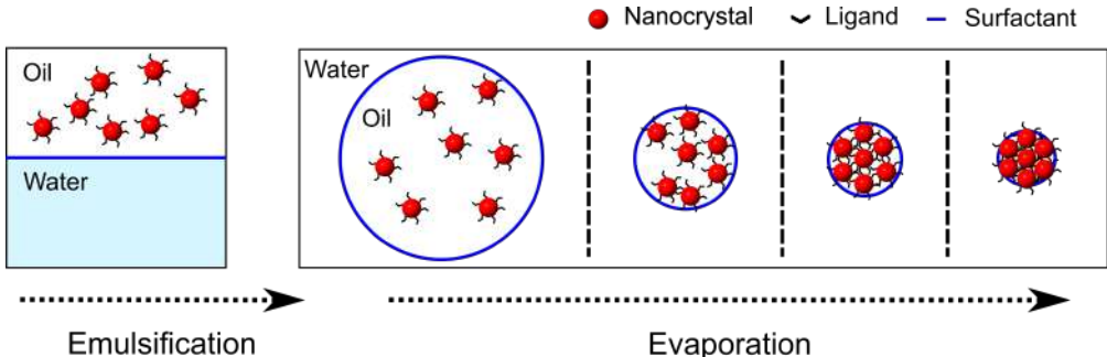
Figure 1: Schematic of the emulsion-templated assembly process. Schematic of the emulsion-templated assembly process. A dispersion of NCs in a hydrophobic volatile solvent is layered on an aqueous solution of surfactant. The emulsification of this two-phase system leads to droplets containing the NC dispersion. As the hydrophobic phase, also known as the dispersed phase, slowly dissolves into the aqueous phase, or continuous phase, the NC volume fraction increases, eventually leading to supercrystal nucleation.
