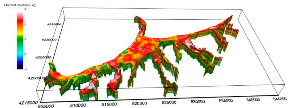
Figure 10. 3D model of the distribution of the logarithm of the electrical resistivity of the BMGWB.
