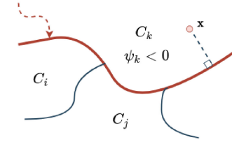
Fig. 4. Graphical interpretation of the misclassification measure. If misclassification measure \psi_k = 0 for a sample \mathbf{x} , then this sample is on the decision boundary \mathcal{B}_k . Otherwise, the absolute value of the misclassification measure defines a distance to the decision boundary and the sign tells the decision: \psi_k < 0 means a sample belongs to the class C_k , else it is misclassified.
