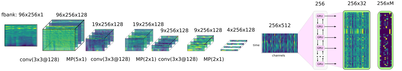
Fig. 3. Multi-label architecture using convolutional recurrent neural network (CRNN). Sequence of convolutions and max-pooling is followed by bi-directional gated recurrent unit (Bi-GRU), which is unfolded on the figure. The output decision layer has dimension of 256 \times M , where M is the number of speech attribute classes ( M = 6 for manner, M = 9 for place or M = 15 for fusion of articulatory attributes). We optimize either binary cross-entropy or MFoM-micro-F1, MFoM-EER objective functions for the same network architecture.
