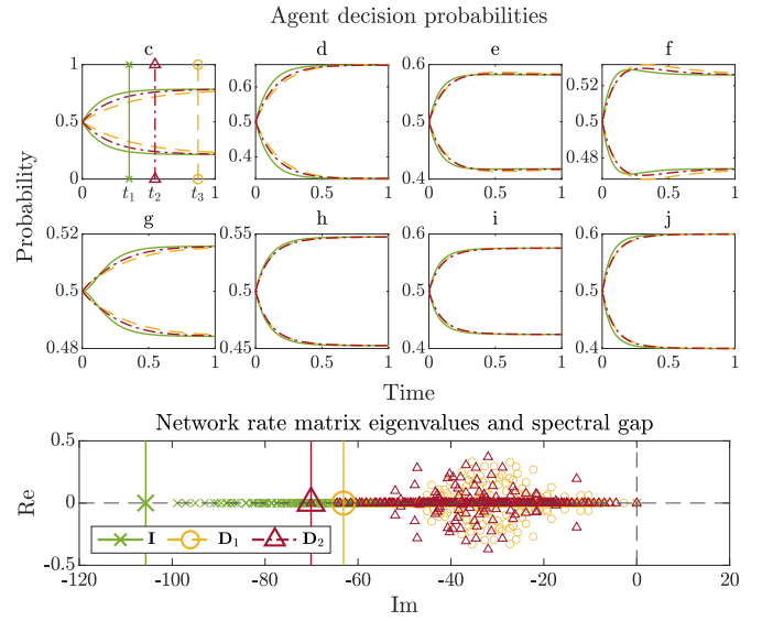
Fig. 3. Agent decision probabilities and eigenvalues.
