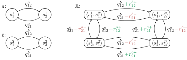
Fig. 2. CTMCs a and b and their network CTMC \mathbb{X} .
