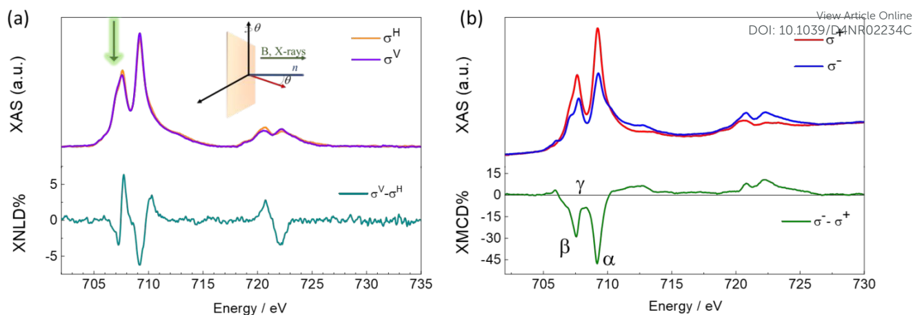
Figure 3 - (a) XNLD and (b) XMCD spectra of \text{Fe}_4\text{SMe} on \text{TiO}_2/\text{Cu} acquired at the Fe L_{2,3} edges. (a) XAS (top) and XNLD (bottom) spectra recorded at \vartheta = 45^\circ , H = 30 kOe, and T = 220 mK. (b) XAS (top) and XMCD (bottom) spectra recorded at \vartheta = 0 , H = 30 kOe, and T = 220 mK. The inset in panel (a) depicts the experimental geometry used for the acquisition of the XAS spectra.
