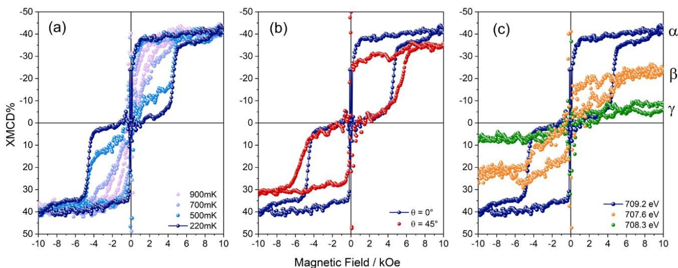
Figure 4 – Magnetic field-dependent XMCD curves acquired (a) as a function of temperature at 709.2 eV and normal incidence ( \vartheta = 0 ), (b) as a function of \vartheta at 709.2 eV and 220 mK, and (c) as a function of photon energy at normal incidence and 220 mK (magnified from -10 to 10 kOe). All data were obtained at the same field sweep rate of 0.2 kOe/s. The measurements at 220\text{mK} , \vartheta=0^\circ , E=709.2\text{eV} is reproduced with dark blue dot plus line along in (a), (b) and (c) and compared with the other measurements where one parameter (temperature (a), angle (b) and energy (c)) is varied.
