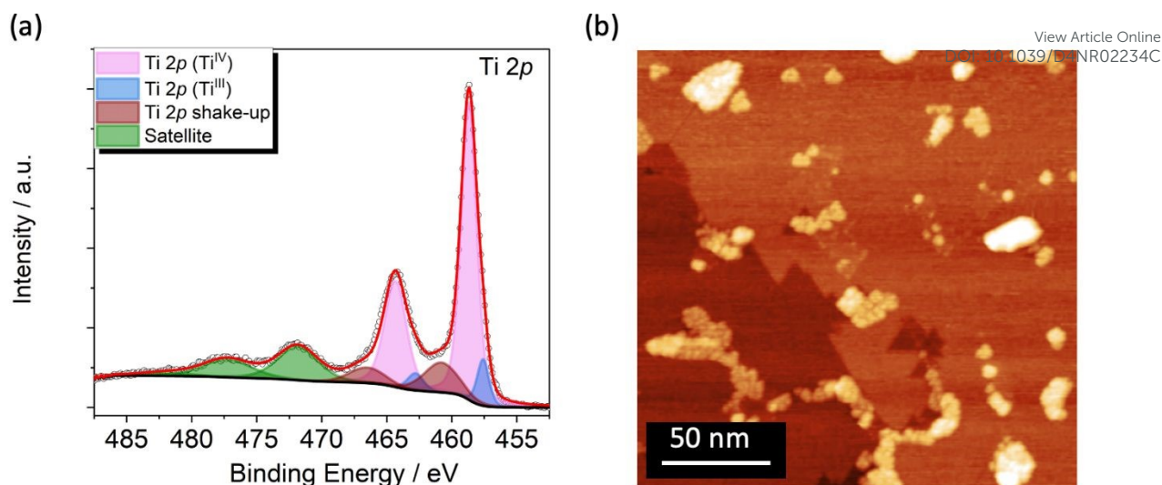
Figure 1- (a) Ti 2p XPS spectrum of the TiO 2 single layer grown on Cu(001) single crystal. (b) STM image of the TiO 2 /Cu surface at RT ( V = 1.5 V, I_t = 150 pA).
