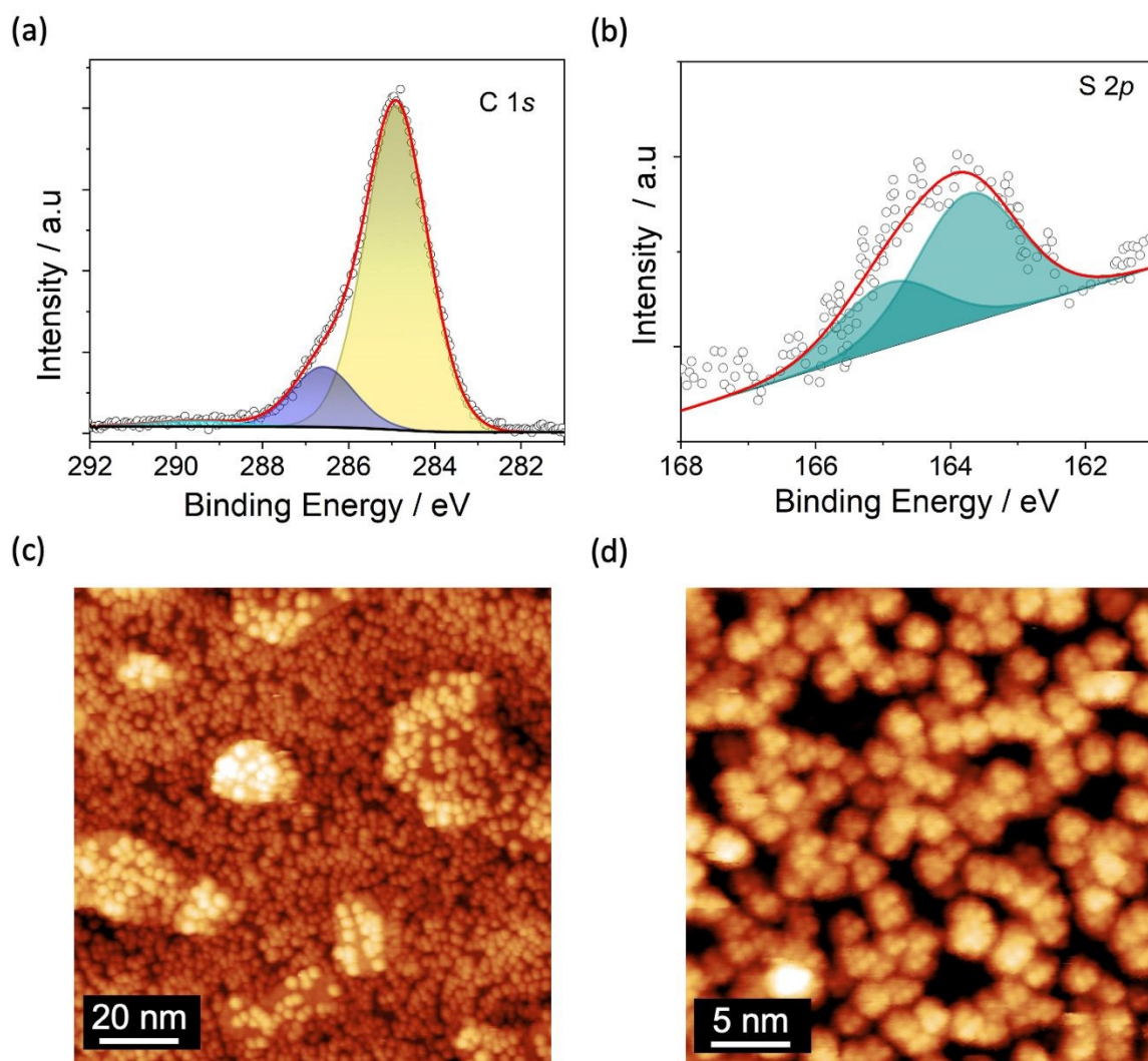
Figure 2 – XPS spectra in the C 1s (a) and S 2p (b) regions after deposition of Fe 4 SMe on TiO 2 /Cu surface. (c) STM image at 30 K of Fe 4 SMe molecules distributed randomly on the TiO 2 /Cu surface ( V = 2.6 V, I_t = 15 pA, 120 \times 120 nm). (d) STM image at 30 K of the Fe 4 SMe layer showing the internal resolution (yellow dots) of single molecules ( V = 2.6 V, I_t = 5 pA, 30 \times 30 nm).
