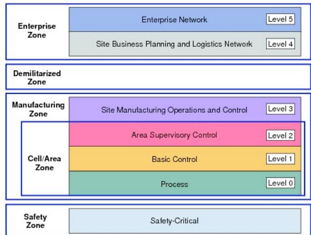
Fig. 1: The Purdue Reference Architecture for ICS [21]
