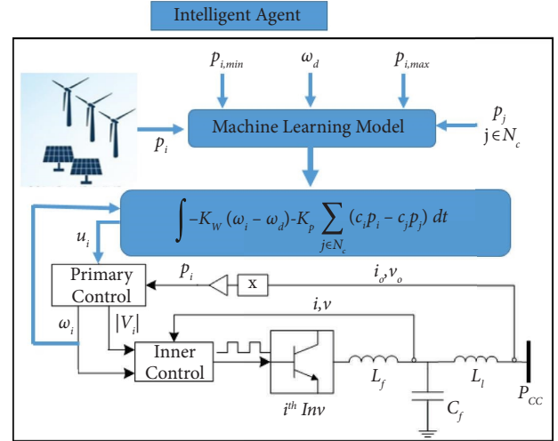
FIGURE 1: Intelligent renewable agent.
