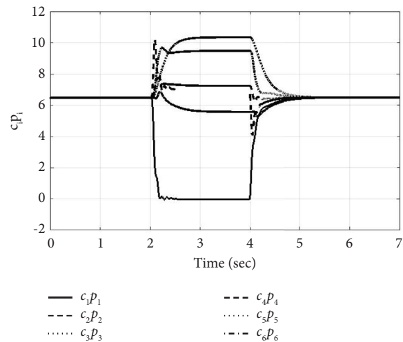
FIGURE 10: Economic dispatch consensus using classical DAI design under node 1 power intermittence.
