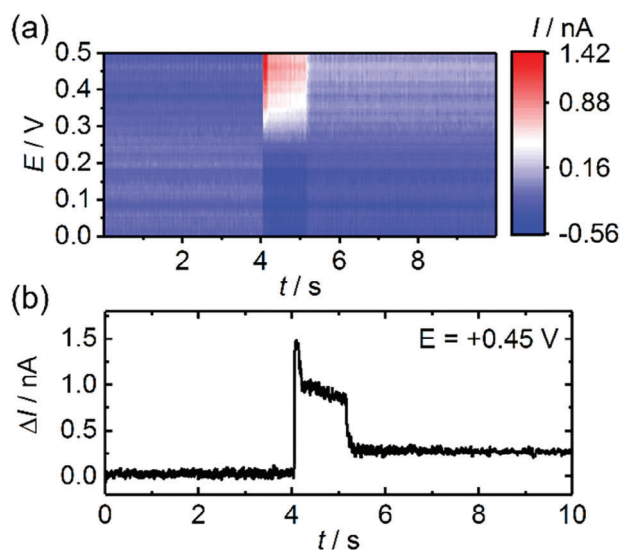
Figure 4. FSCV of FDM at a vdWEdge electrode. a) A color map showing the voltammetric response during the entire measurement cycle. The measurement starts at t = 0 s with only 0.1 M KCl. At t = 4 s, FDM is injected to achieve a final concentration of 0.5 mM. The voltage is continuously scanned in the range of 0 to 0.5 V at a rate of 100 \text{ V s}^{-1} during the entire measurement. Only the forward cycle is shown here. b) A cross-section of the measured voltammetric response in (a), showing the evolution of current at a voltage of +0.45 V. The data are background subtracted using the current response in the first cycle. The potentials are with reference to an Ag/AgCl wire reference electrode.
