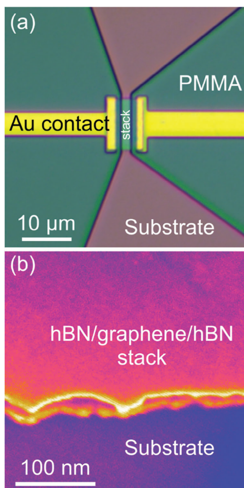
Figure 2. Different views of a vdWEdge device. a) Optical image of a typical device in top-view with the hBN/graphene/hBN stack in between the Au contacts as indicated. b) False-color high-resolution SEM image of the peripheral region of a vdWEdge device, where the two hBN crystals are discernible. The graphene edge lies open in between the edges of these two layers highlighted in yellow.
