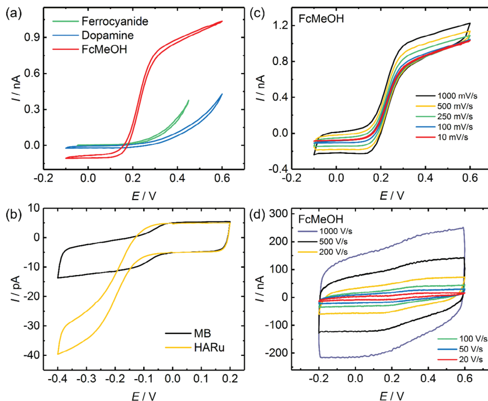
Figure 3. CVs of selected redox-active species at vdWEdge electrodes. a) CVs of species undergoing oxidation: ferrocyanide (0.1 mM), dopamine (1 mM), ferrocenemethanol – FcMeOH (1 mM). b) CVs of molecules undergoing reduction: methylene blue – MB (0.1 mM), hexaammineruthenium – HARu (0.1 mM). c, d) CVs at varying scan rates for the oxidation of FcMeOH (1 mM slow scan, 5 mM fast scan) at a vdWEdge electrode – low scan rates (c) and high scan rates (d). The potentials are measured with reference to a commercial Ag/AgCl (3 M KCl) reference electrode. Scan rate was 100 \text{ mV s}^{-1} in (a) and (b). For dopamine and FcMeOH, a phosphate buffer (pH 6.7, 100 mM ionic strength) was used. The other measurements were performed in 0.1 M KCl.
