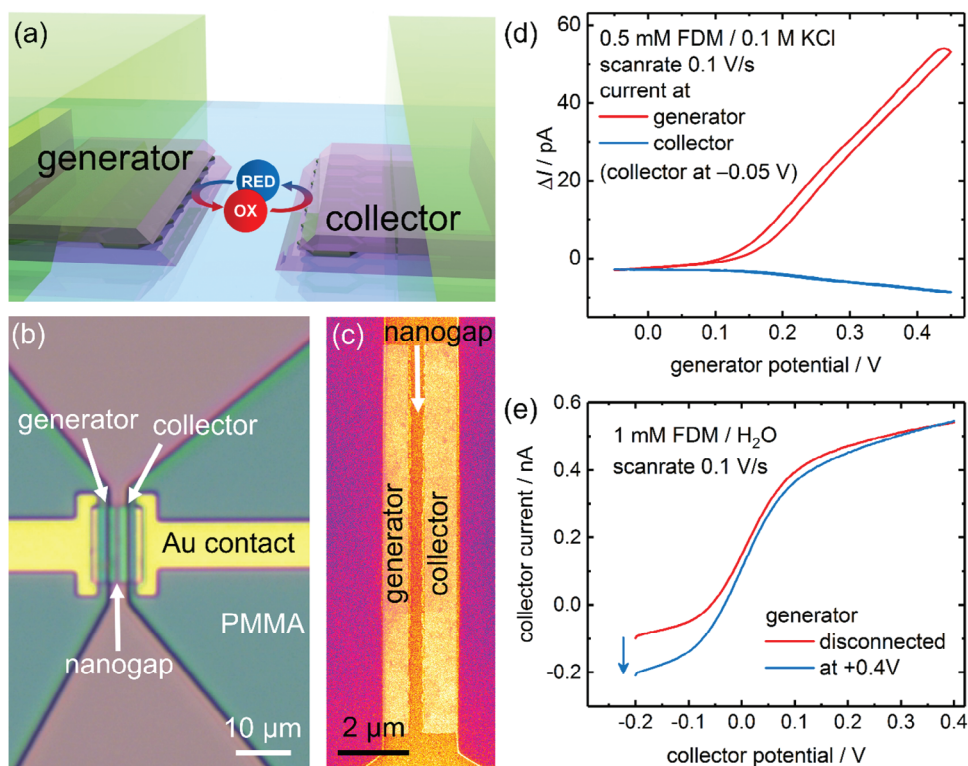
Figure 6. Redox cycling in a vdWEdge nanogap device. a) Schematic of the dual vdWEdge electrode with a nanogap. The scheme shows one example of redox cycling where the collector electrode on the right is maintained at a constant cathodic potential, while the generator electrode potential is scanned in a selected voltage range where oxidation occurs. b) Optical and c) false-color SEM images showing top view of such a redox cycling vdWEdge electrode with a gap of 200 nm. d) CVs obtained in 0.1 M KCl for the redox cycling of FDM with the collector electrode maintained at a potential of -0.05 V as exemplified in (a). e) CVs obtained at the collector electrode in water (without added electrolyte) for the redox cycling of FDM with the generator electrode either disconnected or maintained at an anodic potential. The potentials are measured with reference to an Ag/AgCl wire reference electrode.
