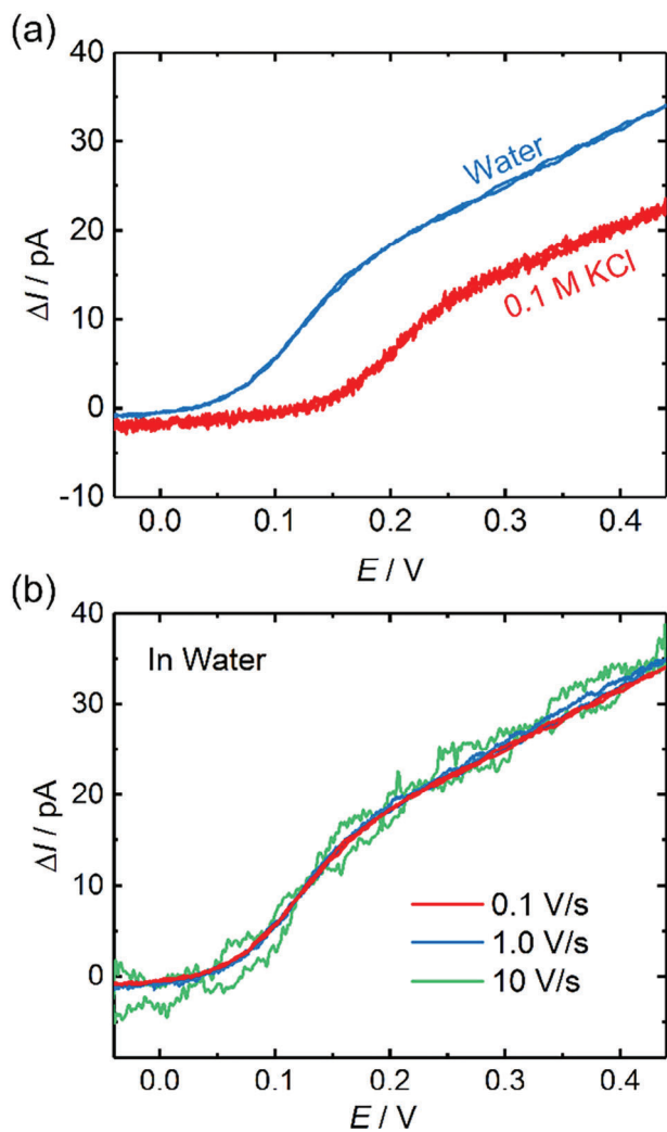
Figure 5. Electrochemistry of 100 \mu\text{M} FDM in water free of supporting electrolyte. a) Comparison of background-subtracted CV measured at a scan rate of 0.1 \text{ V s}^{-1} without added supporting electrolyte (blue curve) to that measured with added 0.1 M KCl (red curve). b) CVs measured at varying scan rates without added supporting electrolyte. The potentials are with reference to an Ag/AgCl wire reference electrode.
