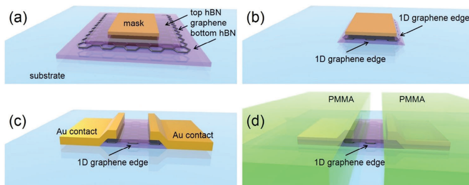
Figure 1. Simplified workflow showing the fabrication of a vdWEdge device. a) An Al hard mask was fabricated on top of the hBN/graphene/hBN stack, which was assembled on top of a SiO 2 /Si substrate by a hot pick-up technique. [34] b) After RIE, the part of the stack unprotected by the mask was etched away. c) After removal of the mask, the Au electrodes were fabricated on the opposite sides of the stack forming contacts to the exposed 1D edges of graphene. d) The contacts were passivated by a PMMA layer such that the remaining 1D edges of graphene were exposed to the environment.
