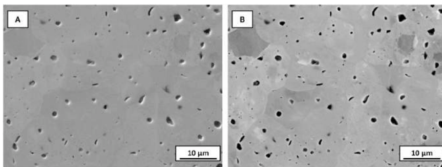
Fig. 3. SEM micrographs of the (\text{Hf}_{0.5}\text{Zr}_{0.5})\text{B}_2 sample produced by SPS (1850 °C) from SHS powders in presence of 1 wt% graphite: A) Secondary and B) back-scattered electron images.
