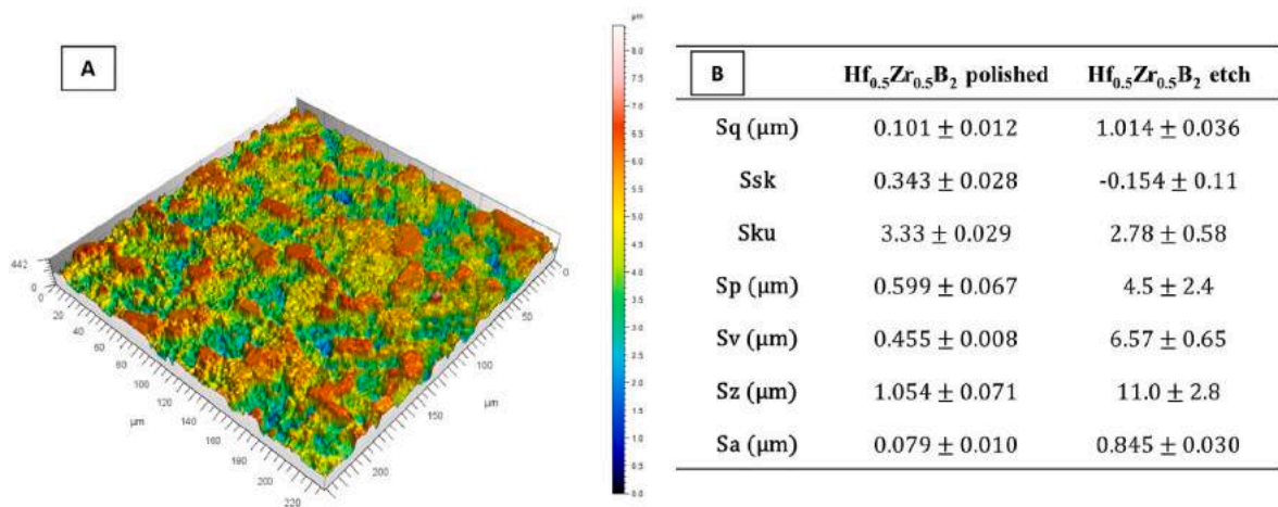
Fig. 9. (a) Areal surface maps of etched surface; (b) Height parameter values evaluated on polished and etched samples.
