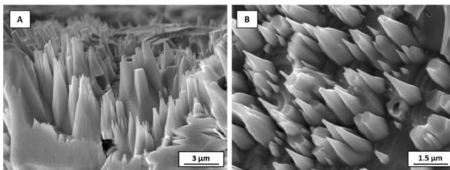
Fig. 7. SEM micrograph of the etched sample, with details of etched morphology at higher magnification. A) SE image obtained from cross-section observation; B) SE image of textured areas.
