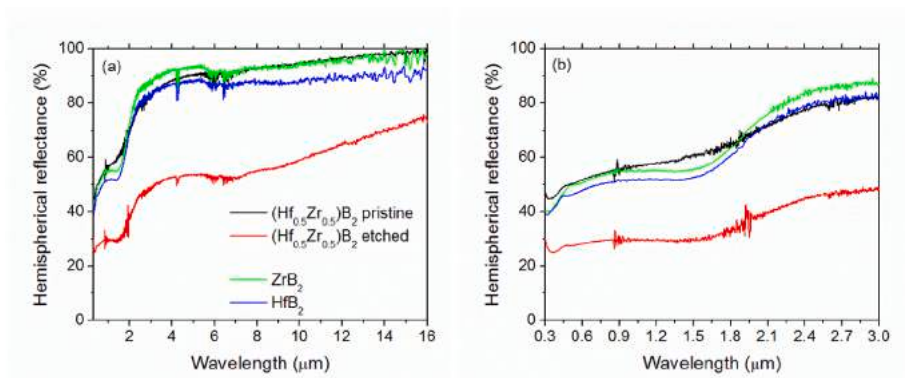
Fig. 10. Hemispherical reflectance spectra of pristine and etched binary borides, and single Zr- and Hf borides, for reference. (a) Full range 0.3–16.0 μm and (b) solar spectrum range 0.3–3.0 μm.
