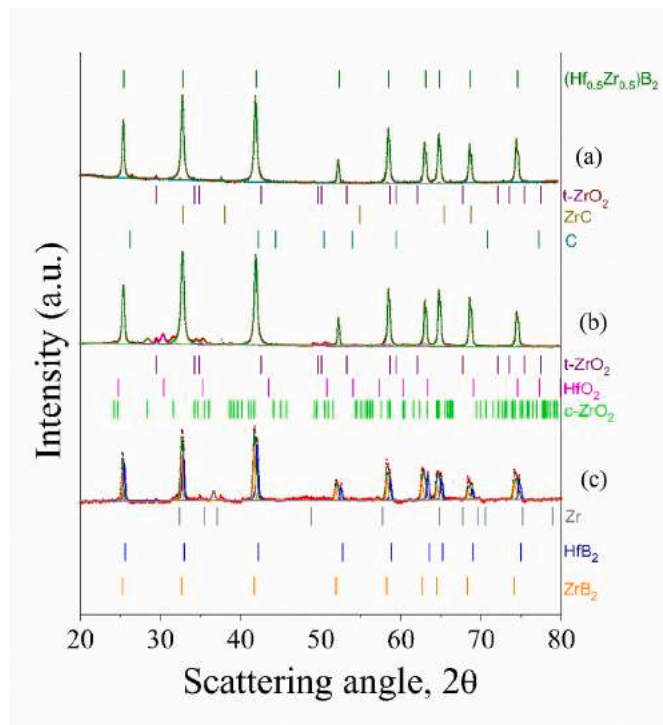
Fig. 1. XRD patterns of SHS (a), and SPS products with no additive at T_D = 1950 °C (b) and in presence of 1 wt% graphite at T_D = 1850 °C (c). Red dots are experimental data, the continuous lines are the calculated best fit.
