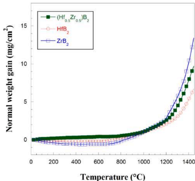
Fig. 2. Comparison of specific weight changes during TGA oxidation test in air of (Hf_{0.5}Zr_{0.5})B_2 sample prepared by SPS ( T_D = 1850 °C, 1 wt%C) in this work as a function of temperature (heating rate equal to 2 °C/min). Literature data of individual diborides ( HfB_2 , ZrB_2 ) are also reported for comparison [18,26].
