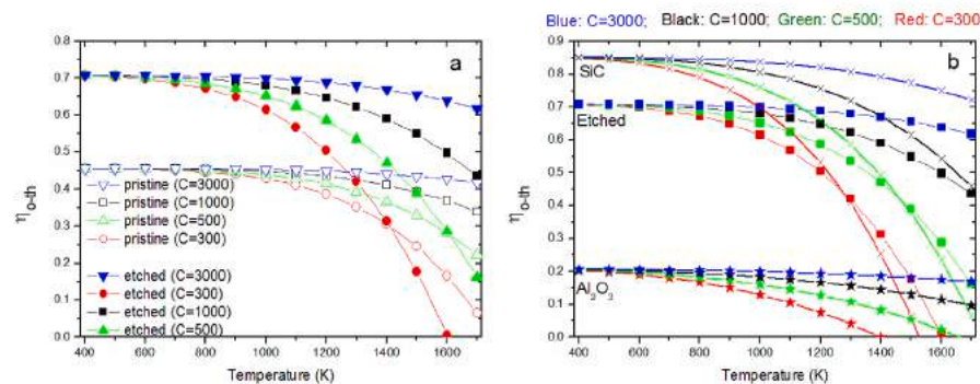
Fig. 13. Opto-thermal efficiency as a function of the temperature. (a) Comparison of the two binary borides. Hollow symbols: untreated sample. Filled symbols: etched sample. (b) Comparison of the etched binary sample to two commercial reference materials (SiC and \text{Al}_2\text{O}_3 ). Meaning of symbols: crosses: SiC; filled squares: etched binary boride; stars: \text{Al}_2\text{O}_3 . The color code is referred to the values of the solar concentration ratio, as explained in legend.
