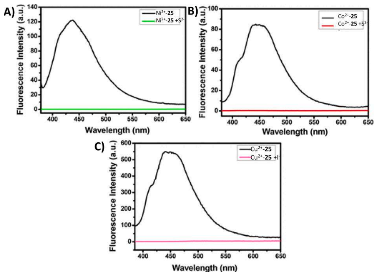
Fig. 31. Fluorescence spectra of metallogels of 25 in DMF with different anions ( \lambda_{\text{exc}} = 355 \text{ nm} ). A) Ni 2+ -25 and Ni 2+ -25 in the presence of S 2- ; B) Co 2+ -25 and Co 2+ -25 in the presence of S 2- ; C) Cu 2+ -25 and Cu 2+ -25 in the presence of I - . Copyright ACS 2018. Adapted with permission from ref [84].
