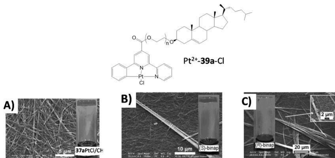
Fig. 43. Visual chiral recognition of (R)- and (S)-binap by metallogel \text{Pt}^{2+} - 39a-Cl / \text{CHCl}_3 (1 wt%) SEM images of A) metallogel \text{Pt}^{2+} - 39a-Cl ; B) metallogel \text{Pt}^{2+} - 39a-Cl + 0.1 equivs. of (S)-binap; C) metallogel \text{Pt}^{2+} - 39a-Cl + 0.1 equivs. of (R)-binap. Copyright Wiley 2011. Reproduced with permission from ref [102].
