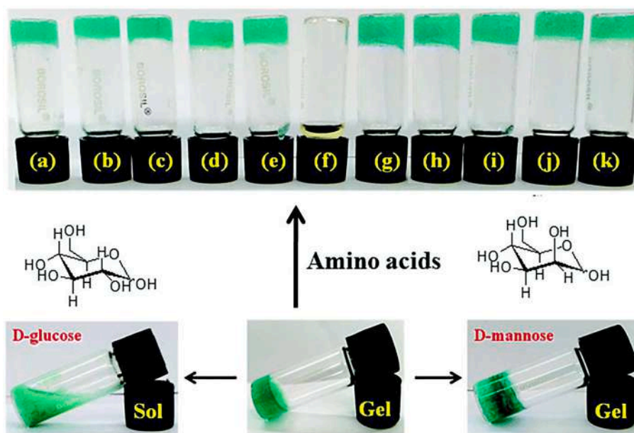
Fig. 41. Pictures of the Cu 2+ -33 metallogel in DMSO/H 2 O (1:1 v/v) in the presence of 2 equivs. of different amino acids and D-glucose and D-mannose (0.03 M) [(a): glycine, (b): L-valine, (c): L-alanine, (d): L-phenylalanine, (e): L-proline, (f): L-cysteine, (g): L-lysine, (h): L-threonine, (i): L-histidine, (j): L-methionine, (k): L-glutamic acid]. Copyright RSC 2018. Reproduced with permission from ref [100].
