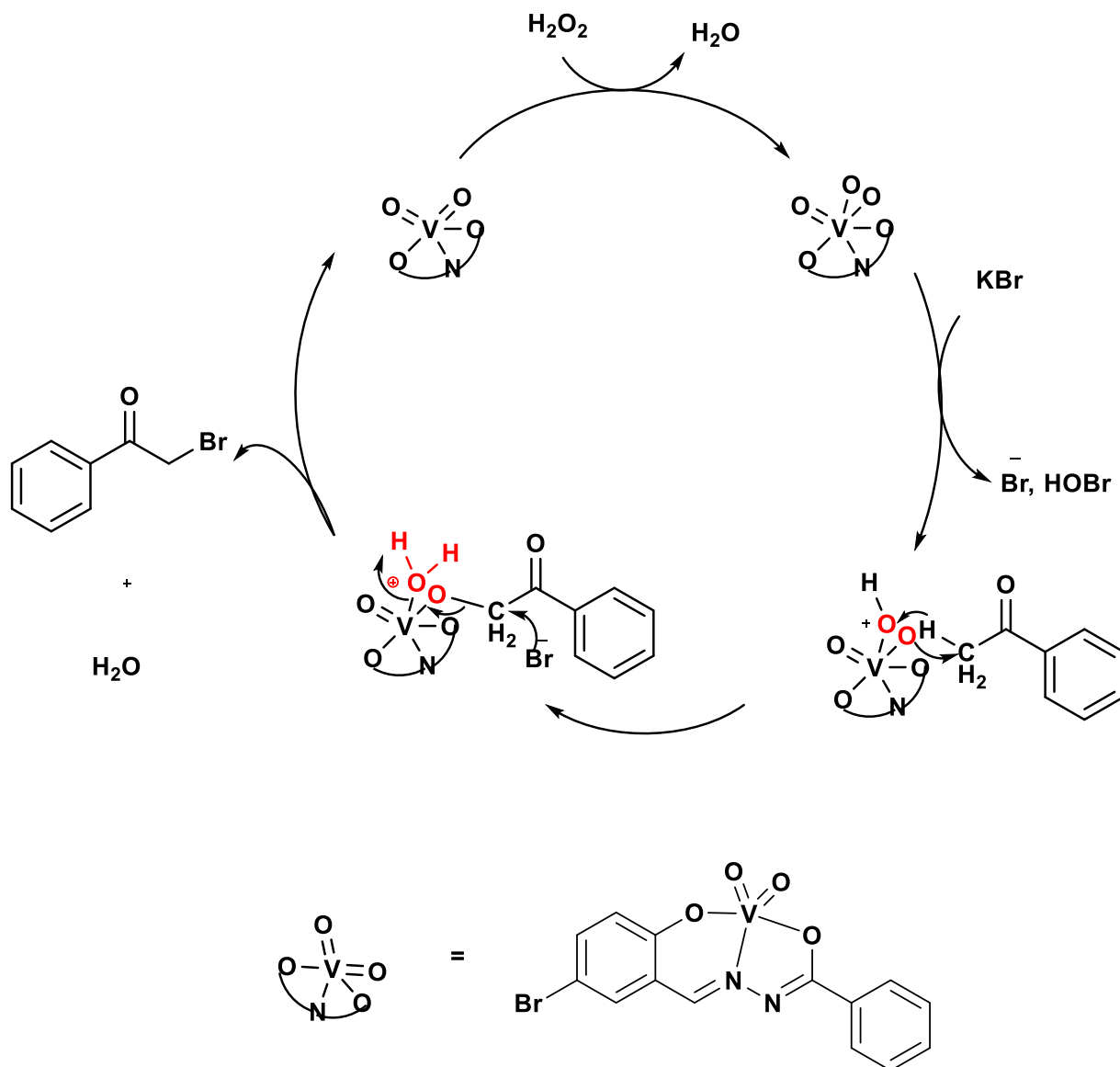
Scheme 1. Possible mechanism for the oxidative bromination catalysed by VO 2 + -56 metallogel. Copyright RSC 2020. Reproduced with permission from ref. [127] (Scheme 2).
