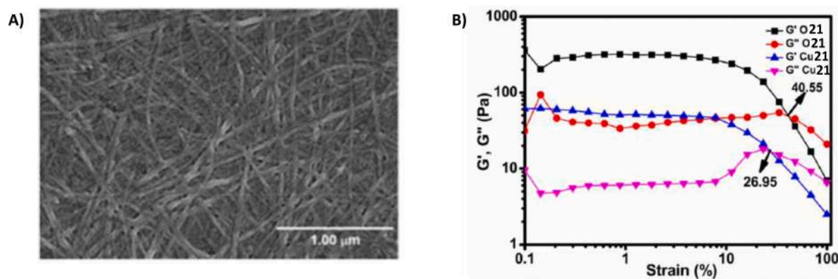
Fig. 27. A) SEM image of the metallogel Cu 2+ -21; B) dynamic strain sweep rheology measurements. Copyright ACS 2020. Reproduced with permission from ref. [82].
