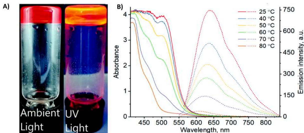
Fig. 11. A) Pictures of the gel formed by \{[\text{Pt}(\text{T})\text{Cl}]\text{Cl}\} in DMSO in the presence and in the absence of UV-light radiation; B) UV-Vis (solid lines) and fluorescence (dashed lines) spectra of the gel formed by \{[\text{Pt}(\text{T})\text{Cl}]\text{Cl}\} (0.6%) in DMSO at different temperatures ( \lambda_{\text{ex}} = 550 and 530 nm for T = 25\text{--}60 °C and T = 70\text{--}80 °C, respectively). Copyright RSC 2020. Reproduced with permission from ref. [66].
