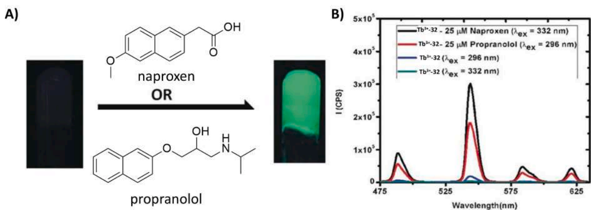
Fig. 39. A) Naked eye (under UV light) switching on of the fluorescence emission of \text{Tb}^{3+} - 32 metallogel in the presence of naproxen or propranolol; B) emission spectra of \text{Tb}^{3+} - 32 metallogel in the presence (black and red lines) or in the absence (blue and green lines) of naproxen or propranolol. Copyright Wiley 2017. Adapted with permission from ref. [99].
