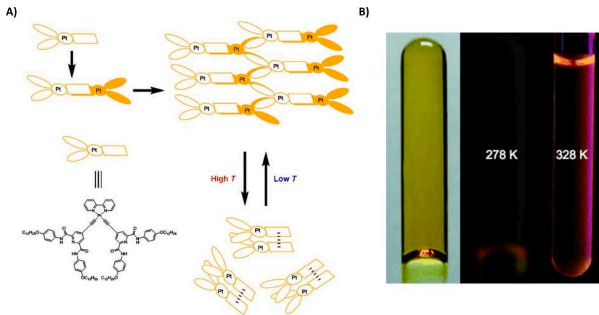
Fig. 12. A) Scheme of excimer formation in the excited state at high temperatures for \text{Pt}^{2+}\text{-9} ; B) \text{Pt}^{2+}\text{-9} in toluene in the viscous form at 328 K (right), in the gel form at 278 K (middle), and at 298 K under the UV-Vis lamp ( \lambda_{\text{ex}} = 365 nm). Copyright Wiley 2012. Reproduced with permission from ref. [67].
