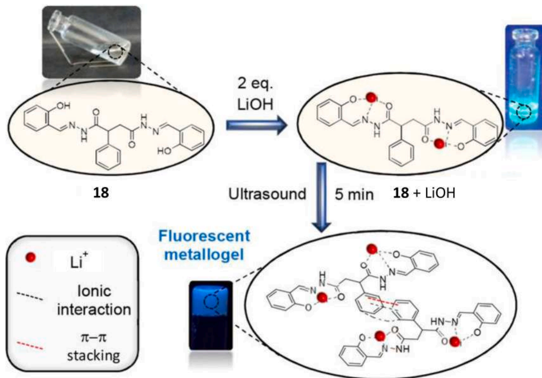
Fig. 24. Schematic pathway for the formation of the \text{Li}^+ -18 metallogel with the associate emission changes. Copyright Wiley 2020. Reproduced with permission from ref. [79].
