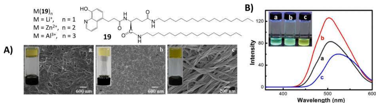
Fig. 25. Structure of gelator 19 ; A) SEM images of (a) \text{Li}^+ -19, (b) \text{Zn}^{2+} -19 and (c) \text{Al}^{3+} -19 xerogels obtained by the corresponding metallogels obtained in THF; B) fluorescence spectra of (a) the \text{Zn}^{2+} -19 metallogel and (b) upon the addition of 1 equiv. of (b) (R,R)- and (c) (S,S)-1,2-diaminocyclohexane in THF ( \lambda_{\text{exc}} = 340 \text{ nm} ). Copyright ACS 2013. Reproduced with permission from ref. [80].
