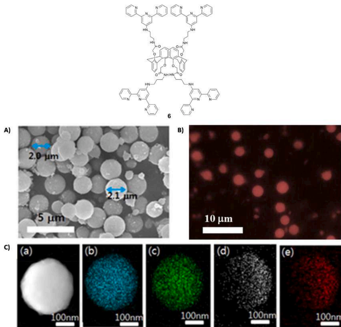
Fig. 8. A) SEM and B) fluorescence microscopy images of Pt 2+ -6 metallogel (1.0 wt%) in DMSO/H 2 O (3:7 v/v); C) energy Dispersive Spectroscopy (EDX) mapping of the Pt 2+ -6 metallogel, (a) bright-field image, (b) platinum, (c) carbon, (d) oxygen, and (e) nitrogen components. Copyright ACS 2014. Reproduced with permission from ref. [65].
