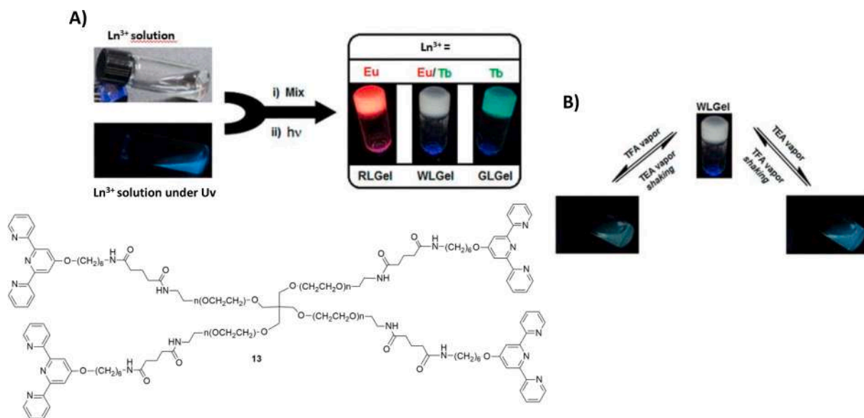
Fig. 17. Chemical structure of gelator 13 . A) Schematic preparation of Ln 3+ coordination-based luminescent metallogels under UV light ( \lambda_{\text{ex}} = 365 \text{ nm} , 3.5 wt% gelator 13 , DMF/MeCN 1:1 v/v); B) stimuli-responsive emission colour changes and phase transitions of white-light metallogel (WLGel): pH-triggered vapochromism. Copyright ACS 2015. Reproduced with permission from ref. [74].
