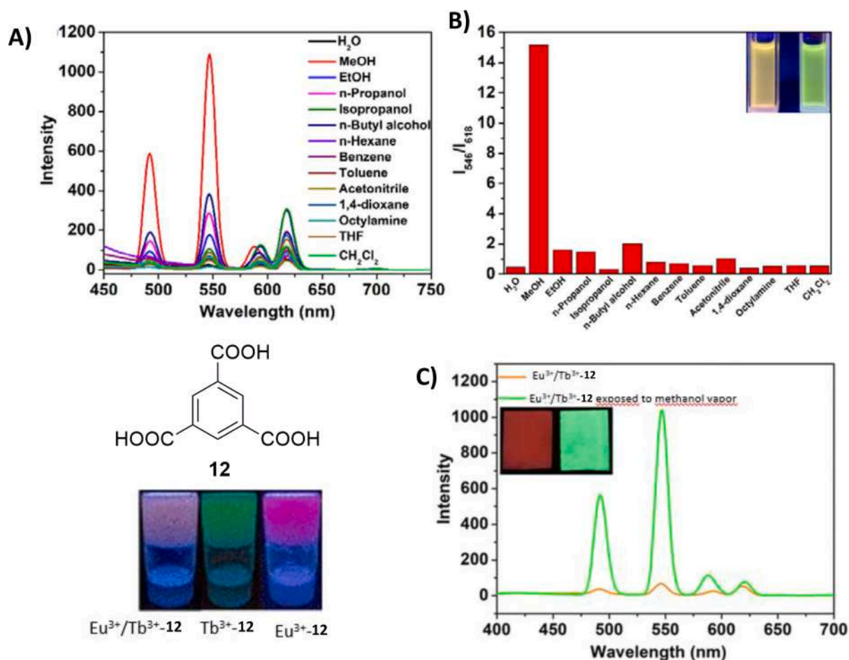
Fig. 16. Molecular structure of 12 and representation of its gels (Eu 3+ - 12 ), (Tb 3+ - 12 ), and (Eu 3+ /Tb 3+ - 12 ) under the UV lamp at 302 nm. A) Luminescence spectra of the Eu 3+ /Tb 3+ - 12 xerogel dispersed in different solvents; B) Histogram of the intensity ratios of Tb 3+ (546 nm) to Eu 3+ (618 nm), inset: different emission visible by naked eye of a dispersed solution in MeOH (right) and EtOH (left) of Eu 3+ /Tb 3+ - 12 ; C) fluorescence spectra of the Eu 3+ /Tb 3+ - 12 paper-based sensor before and after exposing to MeOH vapour, inset: effect of the exposition of the Eu 3+ /Tb 3+ - 12 paper-based sensor to MeOH vapour (right). Copyright ACS 2021. Reproduced with permission from ref. [73].
