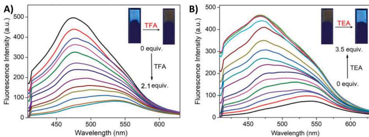
Fig. 38. A) Fluorescence titration of metallogel \text{Al}^{3+} - 31 with TFA ( \lambda_{\text{ex}} = 380 \text{ nm} ) and pictures of \text{Al}^{3+} - 31 and \text{Al}^{3+} - 31 + TFA under 365 nm UV light; B) fluorescence titration of the gelator 31 + TFA with TEA ( \lambda_{\text{ex}} = 380 \text{ nm} ) and pictures of \text{Al}^{3+} - 31 + TFA and \text{Al}^{3+} - 31 + TFA + TEA under 365 nm UV light. Copyright Elsevier 2019. Reproduced with permission from ref [94].
