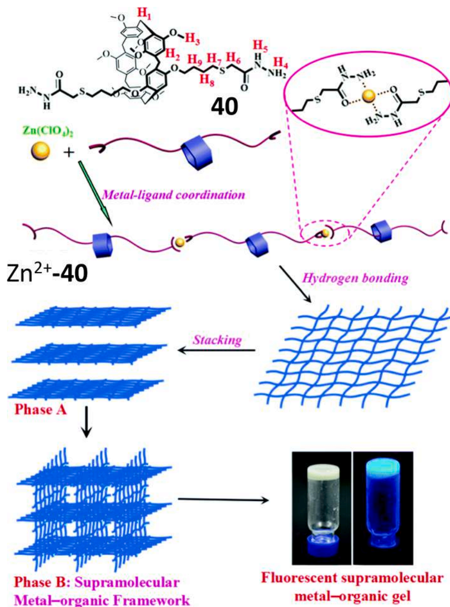
Fig. 44. Representation of the formation of the metal-organic gel of Zn 2+ -40. Copyright RSC 2018. Reproduced with permission from ref. [104].
