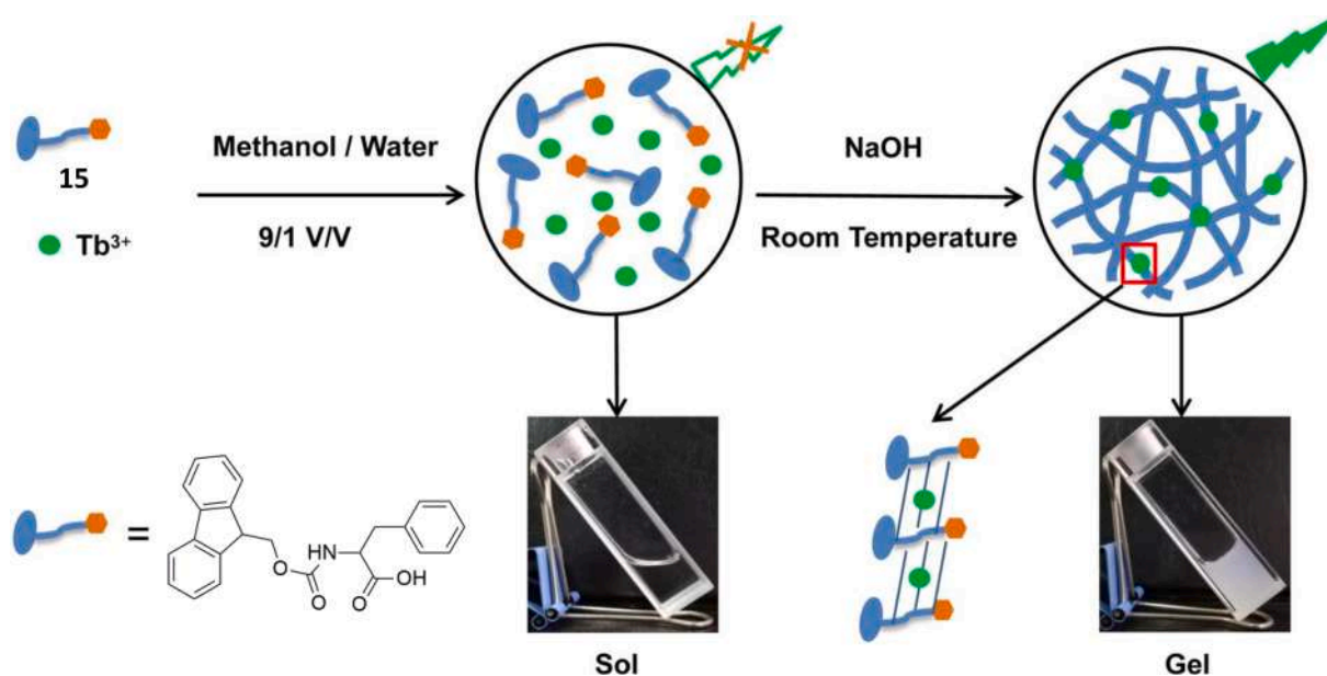
Fig. 19. Scheme of the \text{Tb}^{3+} - 15 gel formation. Copyright Elsevier 2019. Reproduced with permission from ref. [76].
