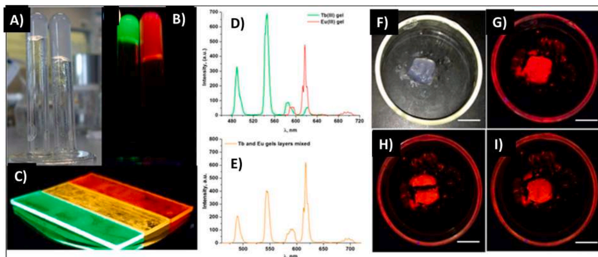
Fig. 15. Eu 3+ and Tb 3+ gels of 11 A) in day light; and B) under UV light; C) luminescence of Eu 3+ , Tb 3+ , and Eu 3+ /Tb 3+ gels of gelator 11 on quartz plates; D) Eu 3+ , Tb 3+ ; and E) Eu 3+ /Tb 3+ - 11 mixed gel luminescence spectra at 25 °C ( \lambda_{\text{ex}} = 275 nm); F – I) healing experiment of Eu 3+ - 11 gel with F) Eu 3+ gel under day light, G) under UV light, H) gel after being cut in half, and I) self-healing properties of the gel (scale bars, 1 cm). Copyright ACS 2015. Reproduced with permission from ref. [72].
