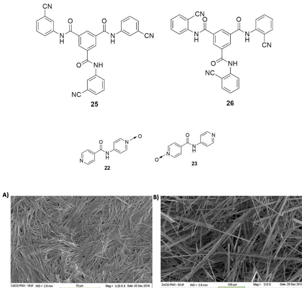
Fig. 29. SEM images of A) xerogels of \text{Cd}^{2+} - 22 in \text{H}_2\text{O} at 3.7 wt%; and B) xerogels of \text{Zn}^{2+} - 22 in DMF/ \text{H}_2\text{O} (1:1 v/v) at 2.8 wt%. Copyright Taylor and Francis 2020. Reproduced with permission from ref. [83].
