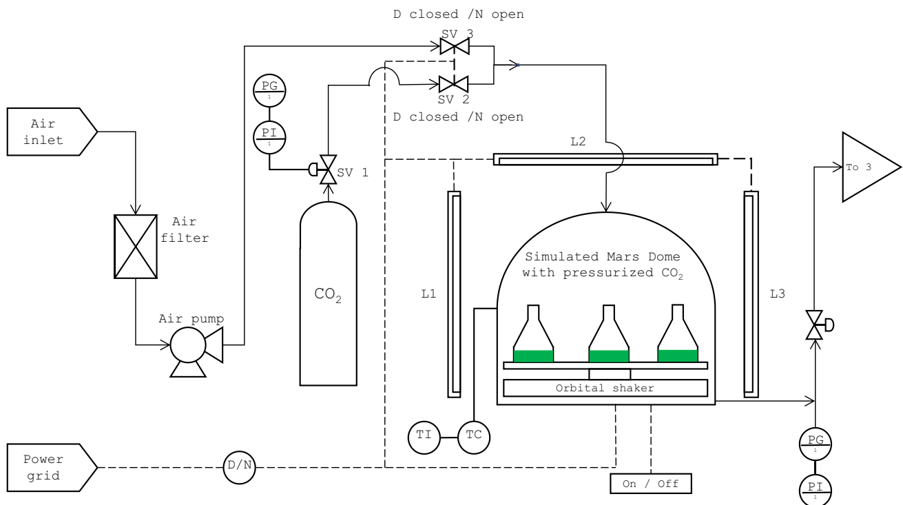
Fig. 2 Scheme of the experimental apparatus adopted to simulate the pressurized Martian domes hosting the process by Cao et al. [22] on Mars
