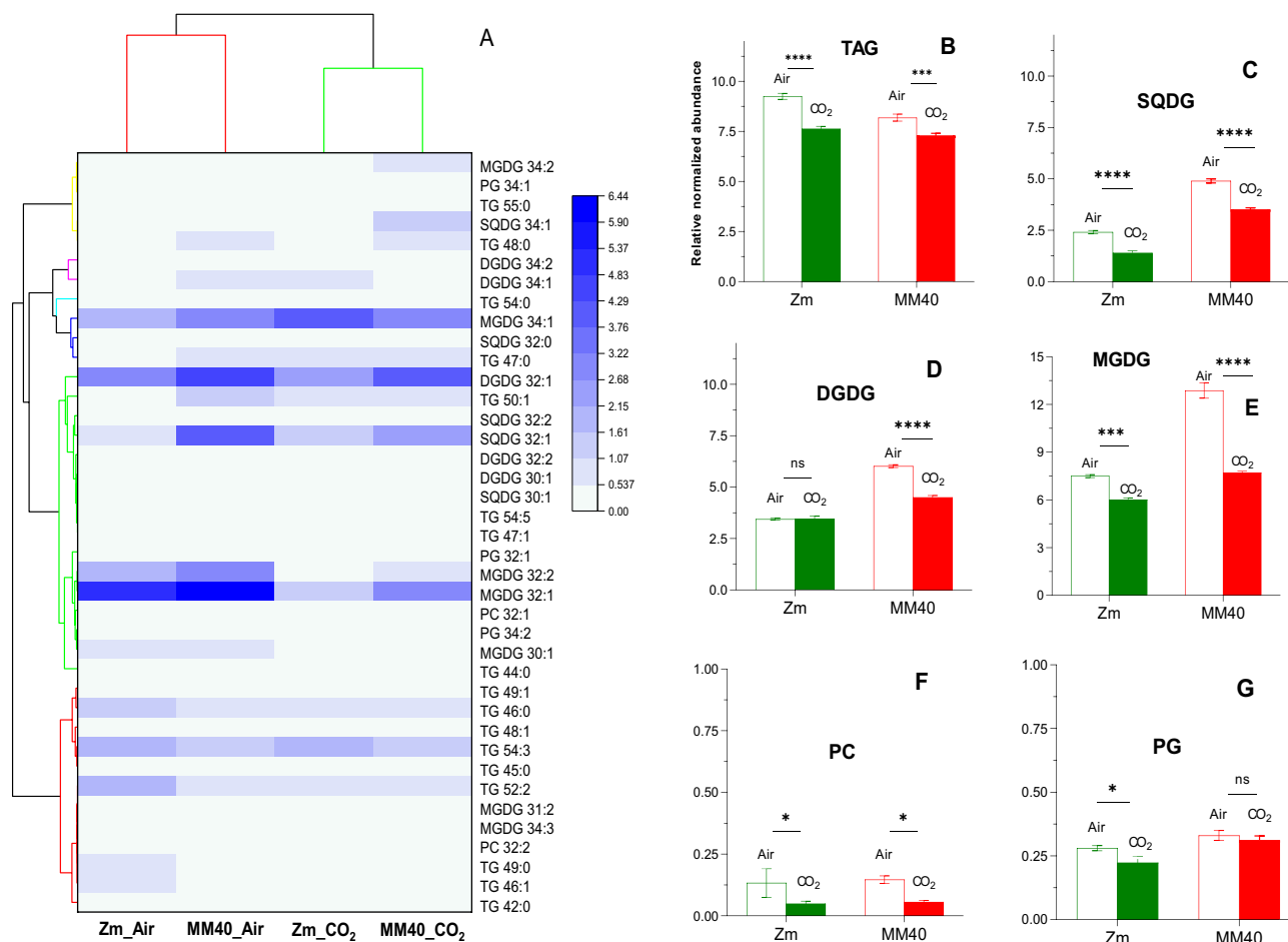
Fig. 7 Heatmap of each lipids compound found (A) and relative contents of TAG, SQDG, MGDG, DGDG, PC and PG (B–G) in the biomass of Synechococcus nidulans grown in different media and atmospheric conditions ( n=3 ). MM: Martian medium, TAG: triglyceride,
