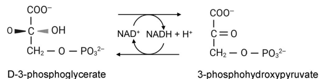
SCHEME 1 The reversible reaction catalyzed by PHGDH.
