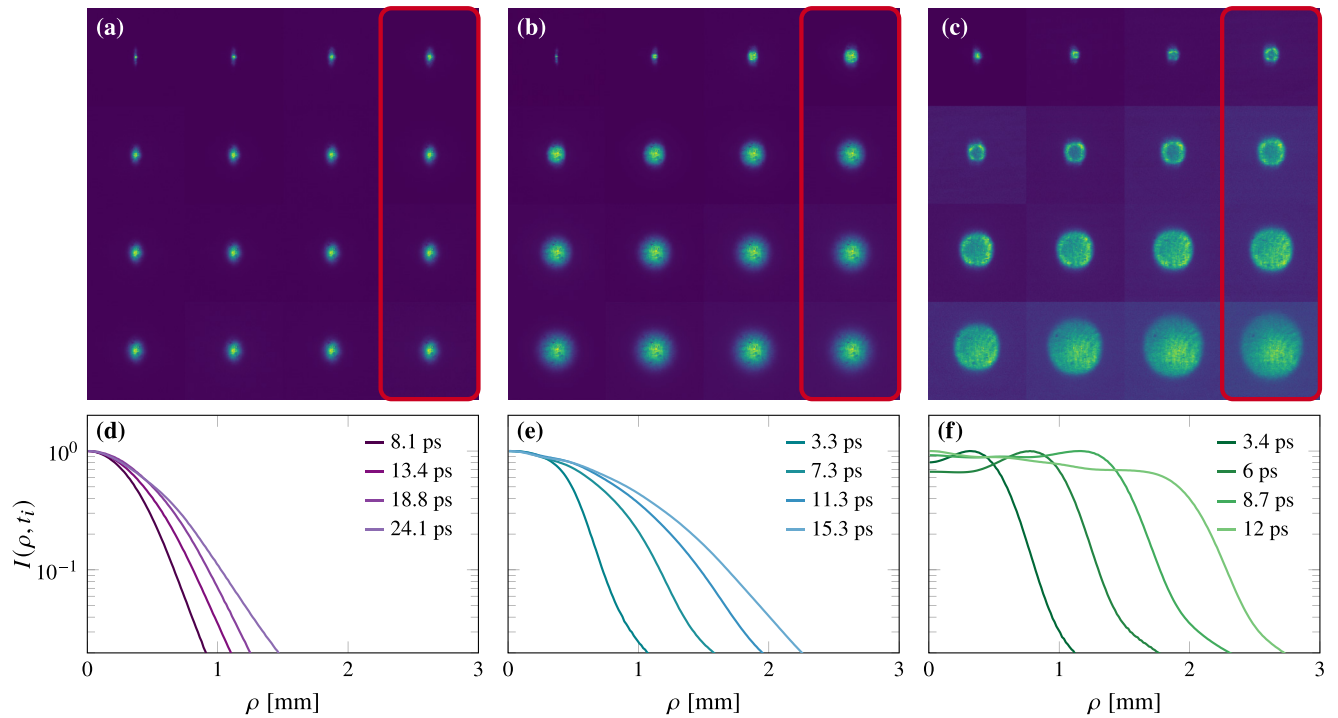
FIG. 2. (a)–(c) Transmitted profiles recorded at different times t_i for three 100- \mu\text{m} -thick samples with different turbidity (samples A, B, and C in order of decreasing turbidity from left to right). Each frame covers the same area of 7.4 \times 7.4 \text{ mm}^2 and is normalized to its maximum value. Time delays between consecutive frames are \Delta t = 1.33, 1.0, and 0.67 \text{ ps} , respectively, for the three cases. (d)–(f) Representative radially averaged profiles corresponding to the highlighted frames. A time-evolving intensity profile is visible for the least scattering sample C: The spatial distribution of light evolves from a ring-shaped profile towards a top-hat-like distribution, showing one of the typical hallmarks of non-self-similarity.
