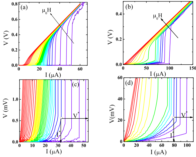
Fig. 2. (a) Representative of I - V curves of the microstrip D2 at T = 2 K in different magnetic fields from 10 mT to 4 T. (b) The same as panel (a) for the microstrip D10 in different magnetic fields from 10 mT to 5 T. (c) Enlarged plot in the low-voltage regime of panel (a) to show the nonlinear conductivity regime and the instability jumps. The point marked on these plots is denoted by coordinates I^* and V^* , representing the instability current and voltage, respectively. (d) Enlarged plot in the low-voltage regime of panel (b).
