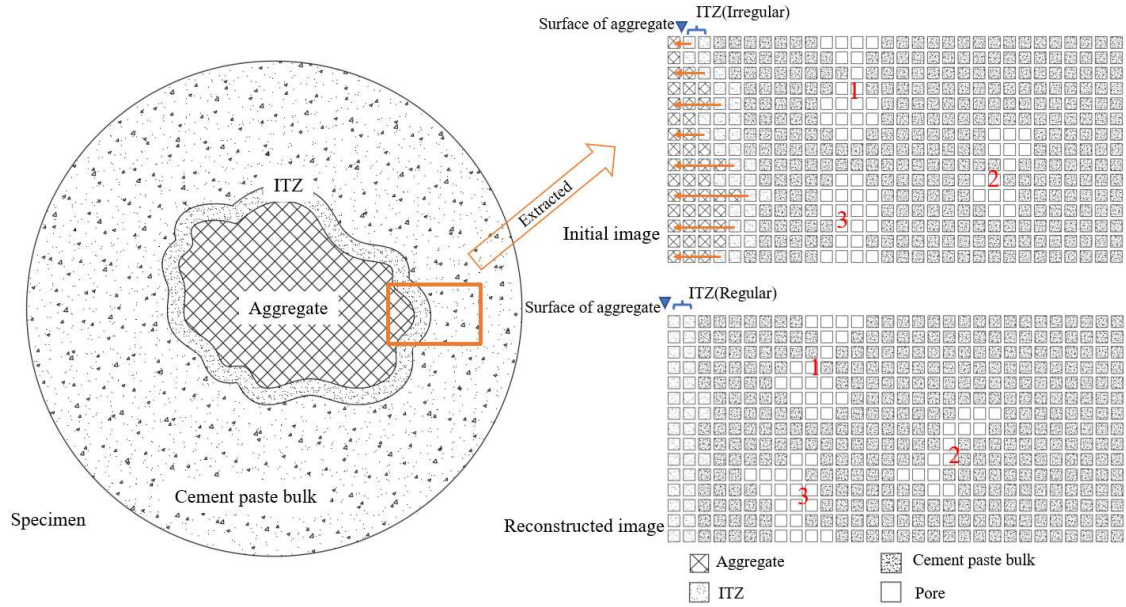
Figure 4-32 Schematic of reconstruction in one single slice
