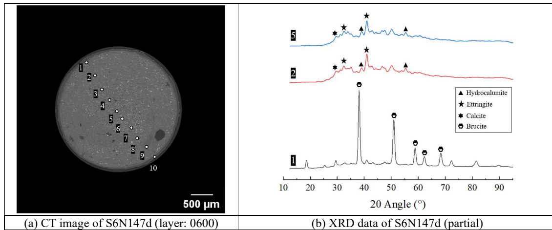
Figure 4-17 CT-XRD result of non-carbonated specimen after 147 days seawater immersion (S6N147d)
