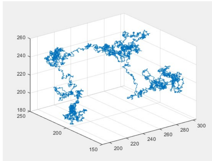
Figure 3-11 Trajectory of single walker in free space ( M = 10000 )
